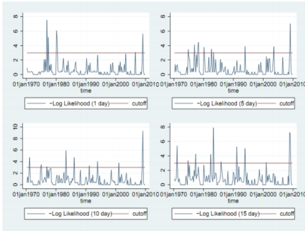
Figure 1.2: This graph reports the log p-values (multiplied by negative unity) of the sequence of tests for each non-overlapping 60 (business) day window to identify clustering at 1, 5, 10 or 15 day horizons when the null is that the layoff announcements are distributed uniformly over each 60 day window.
