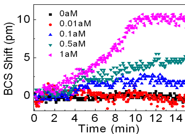
Figure 4.16.— The resonance shift induced by BSA molecules adsorbed on the sensor surface from BSA concentrations of 0aM (pure DI water), 0.01aM, 0.1aM, 0.5aM and 1aM BSAs were injected into the microfluidic channel. The sensor was regenerated with Sodium dodecyl sulfate (SDS) between different concentrations. We hypothesize that the discrepancies in the 1aM response between the current figure and Fig. 3(b) were likely due to inconsistency the surface functionalizations, as well as insufficient regeneration of the sensor between each experiment.
