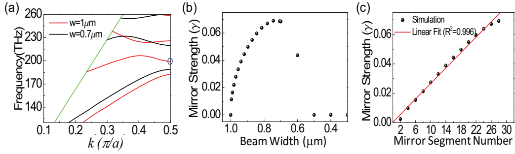
Figure 3.9.— (a) TE band diagram for an air-mode nanobeam cavity. Hole radii r = 100\text{nm} , a = 330\text{nm} , b=1\mu\text{m} (red) and b=0.7\mu\text{m} (black). (b) Mirror strengths for different beam widths. (c) Linearization of mirror strengths after quadratic tapering the beam widths.
