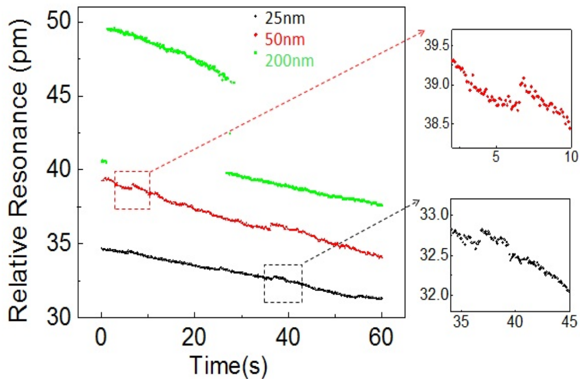
Figure 4.8.— The discrete resonance jumps indicate the detection of single nanoparticles. Polystyrene particles of 25nm, 50nm, 200nm were delivered to the sensor through the fluidic channel.
