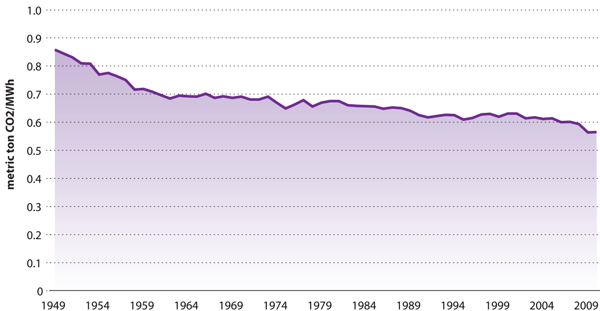
FIGURE 1 U.S. Electricity Generation Carbon Dioxide Emission Intensity, 1949–2010
