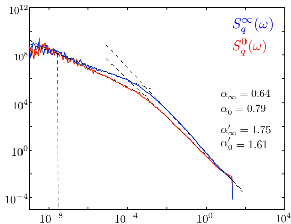
FIG. 7. The structure factors S_q^\infty(\omega) ( T = \infty , blue) and S_q^0(\omega) ( T = 0 , red) are plotted simultaneously, for initial bias \eta_i = 0 , disorder strength D = 3 , system size L = 15000 , and q = 2\pi/160 . The powers \alpha' and \alpha are also indicated for the two cases with the corresponding subscripts. They approximately satisfy the respective scaling relations for zero and infinite temperature cases.
