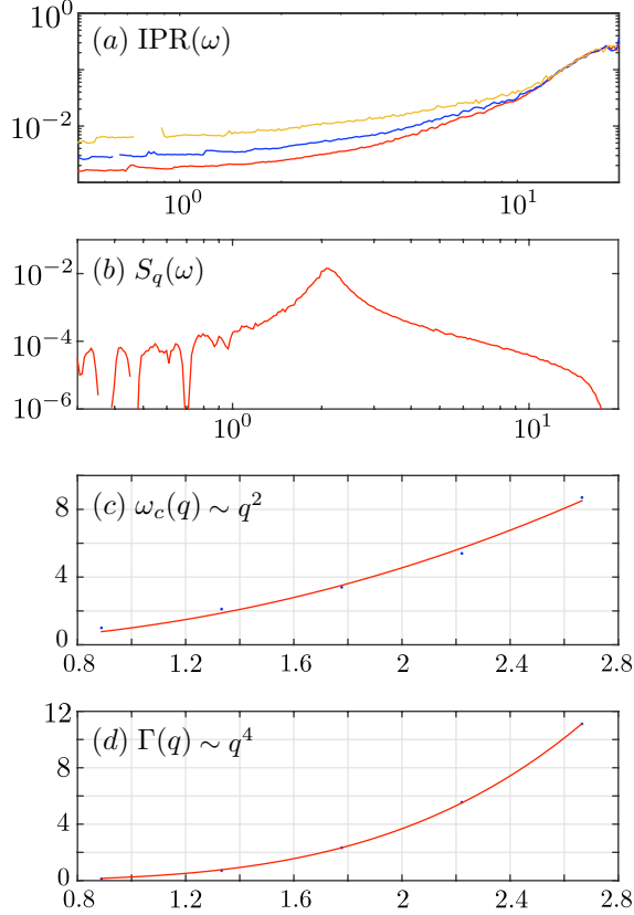
FIG. 19. (a) The inverse participation ratio decreases to zero in the thermodynamic limit [seen by scaling with system sizes 20 \times 20 (yellow), 30 \times 30 (blue) and 40 \times 40 (red)]; (b) spin-wave peak seen in the structure factor S_q(\omega) ; (c) the peak occurs at frequency \omega_c(q) \sim q^2 (red line fit corresponds to q^{2.1} ); (d) the width (calculated as inverse height of the peak) scales as \Gamma(q) \sim q^4 (red line fit corresponds to q^{3.95} ).
