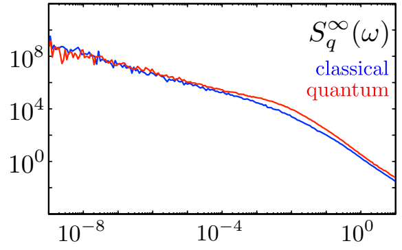
FIG. 20. Infinite-temperature S_q^\infty(\omega) for classical spins of magnitude |\vec{S}| = 1/2 is plotted (blue) and compared with the quantum result (red) at infinite temperature. L = 15000 , D = 3 , \eta_i = 0 .
