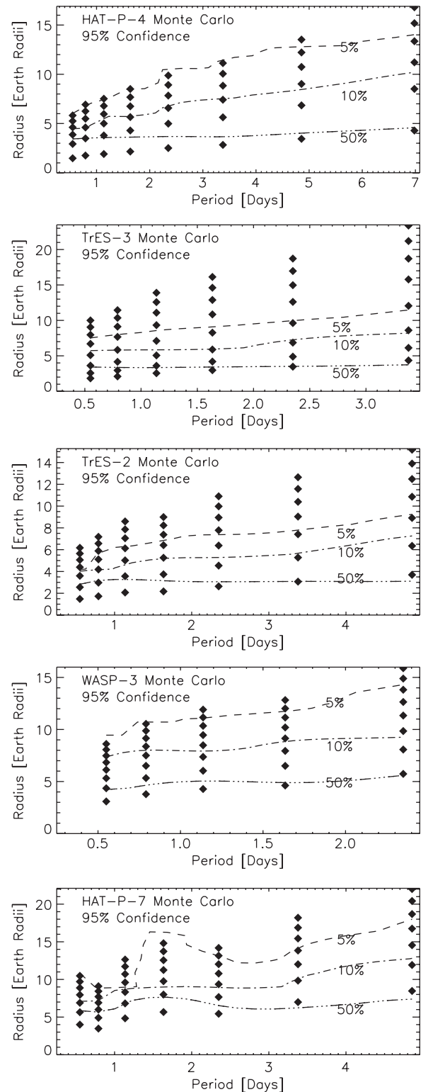
Figure 3. Constraints on radius from the Monte Carlo analysis. For each point in radius and period, we create 75 light curves with random orbital phases, inject them into the EPOCH residuals, and attempt to recover them blindly. The diamonds indicate the grid of radii and periods at which we evaluate our sensitivity; the contours are produced by interpolating between these points. The contours indicate the relative error in radius (absolute value of recovered— \text{injected}/\text{injected} radius) that encloses 95% of the results.
