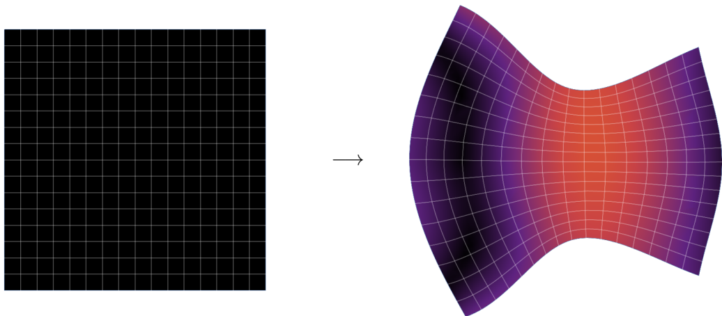
FIGURE 2.1: The mapping illustrated above is quasiconformal. Lighter colors indicate greater local dilatation. Note that the dilatation is greatest where squares are mapped to elongated rectangles.
