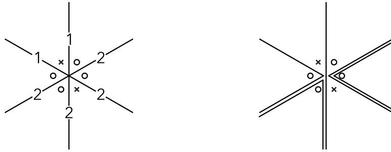
(A) An even integral train track
