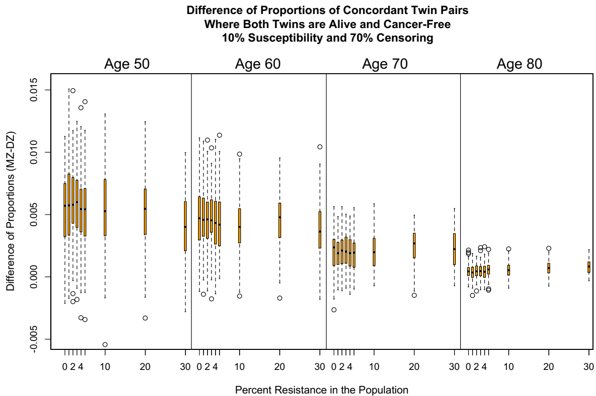
Figure A.9: Concordant twin pairs where both twins are alive and cancer-free by age with 70% censoring. Simulation results based on 79, 520 MZ twins and 123, 348 DZ twins with 70% censoring and 10% susceptibility. Differences in proportions of concordant MZ and DZ twin pairs that are alive and cancer-free, as we vary levels of resistance, across different age groups (50, 60, 70, 80). Results are based on 100 data generations.
