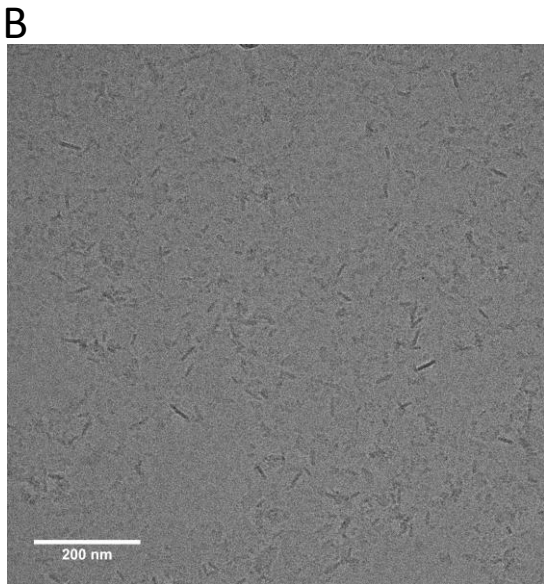
Figure 4.6: Production of CCR5 Nanodiscs. (A) Nanodiscs (Nd) were reconstituted in solution (50 \mu L) at the ratio of 7mM brain:100 \mu M MSP1E3D1 solution and purified via Superose 6 size-exclusion chromatography. Fractions were run on SDS-PAGE and silver stained (above) or immunoblotted with anti-strep antibody (below). (B) Cryo-TEM (120kV) of CCR5 Nanodiscs. Image is representative of >1500 images.
