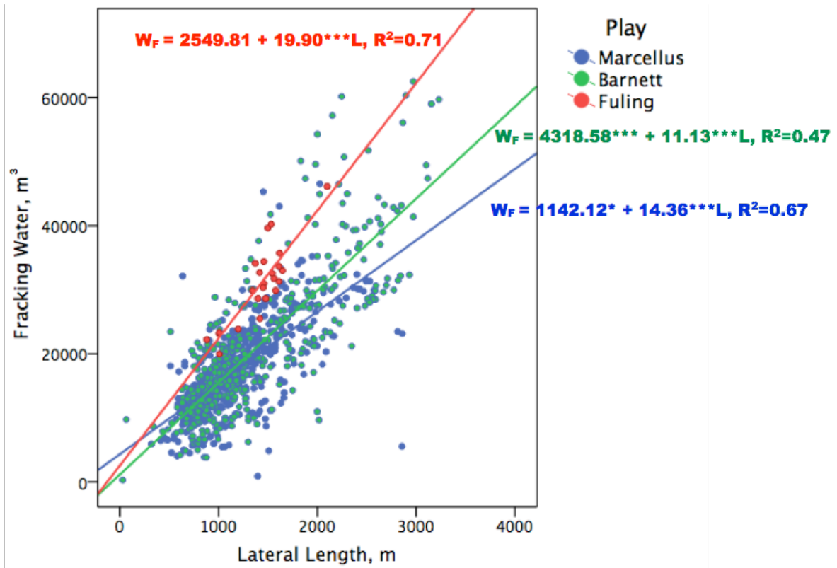
Figure 2. Curve fitting for use of water for fracking in the Marcellus, Barnett, and Fuling plays.
