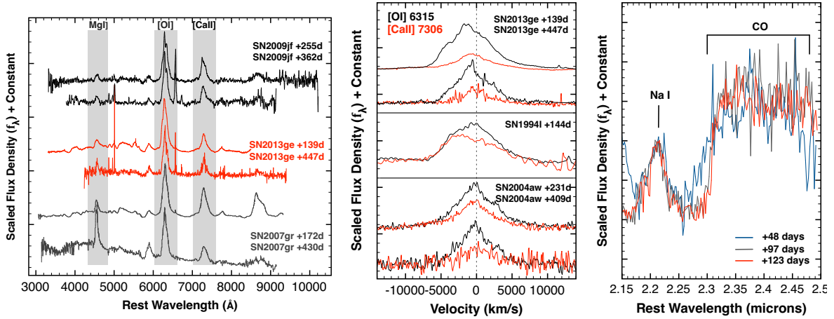
Figure 4.15.— Left: A comparison between the nebular spectra of SN 2013ge, SN 2007gr, and SN 2009jf at multiple epochs. At \sim 150 – 250 days, all have a Mg I] \lambda 4571 to [O I] \lambda \lambda 6300, 6364 ratios of \sim 0.15 . However, by \sim 450 days, the ratio in SN 2007gr has grown substantially to \sim 1 , while it has remained relatively constant in both SN 2013ge and SN 2009jf. Center: Nebular line profiles of SN 2013ge in comparison to SN 1994I and SN 2004aw at a variety of epochs. By late times the [O I] feature in SN 2013ge more closely resembles the peaked structure observed in SN 2004aw. Right: The CO band-head observed in SN 2013ge at three epochs. We observe evolution of the profile between +48 and +97 days. References: SN 2009jf (Valenti et al. 2011), SN 2007gr (Chen et al. 2014), SN 2004aw (Taubenberger et al. 2006), SN 1994I (Filippenko et al. 1995).
