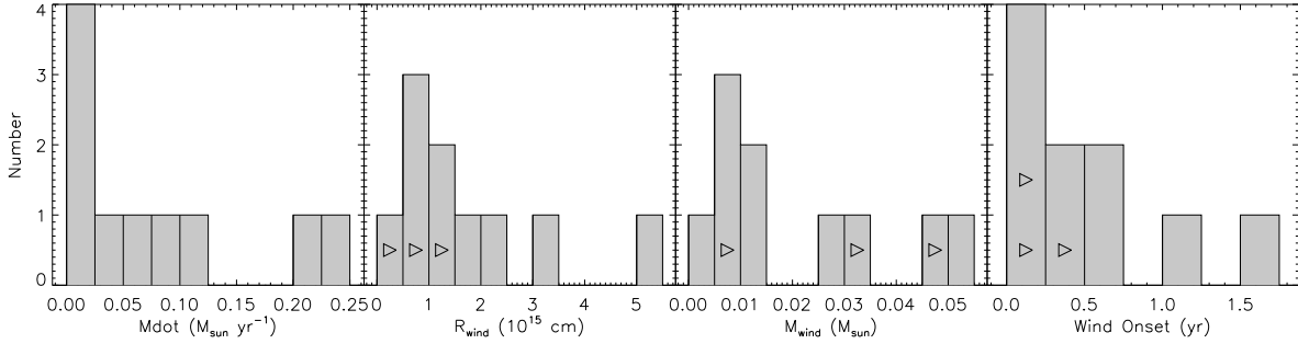
Figure 3.24.—: Histograms of the physical parameters derived for the mass-loss region surrounding each object in the case of a shock breakout from a dense, optically thick, wind. Panels 1,2,3 and 4 display the mass-loss rates inferred from the explosion, the outer radius of the region of dense mass-loss, the total mass contained in the region of dense mass-loss, and the inferred time for the onset of the mass-loss (prior to the main explosion), respectively. Both the mass-loss rates (panel 1) and wind onset times (panel 4) listed assume a wind velocity of 1000 \text{ km s}^{-1} (as measured from a potential CSM absorption in the spectrum of PS1-12bv). The results scale linearly for other assumed velocities.
