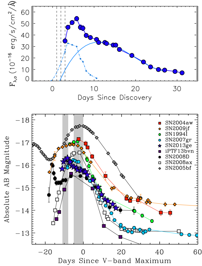
Figure 4.6.—: Top : Example decomposition of the u-band light curve into two components. This should be taken as representative only as we do not constrain the rising behavior of the second component. Dashed vertical lines represent our first three epochs of spectroscopy, which occur on the early rising portion of the first light curve component. Bottom : Comparison of the u-band light curve of SN 2013ge to other stripped core-collapse SN. Shaded regions highlight the time of maximum for both components of SN 2013ge. Most events peak on a timescale similar to that observed for the second component in SN 2013ge. The light curve of SN 2009jf shows a plateau that may be indicative of an early component similar to that observed in SN 2013ge. References : SN 2005bf (Folatelli et al. 2006), SN 2004aw (Taubenberger et al. 2006), SN 2009jf (Valenti et al. 2011), SN 2007gr (Hunter et al. 2009), SN 2008ax (Pastorello et al. 2008), SN 2008D (Soderberg et al. 2008), iPTF 13bvn (Fremling et al. 2014; Cao et al. 2013). Photometry for all objects was converted to the AB system zeropoint before plotting.
