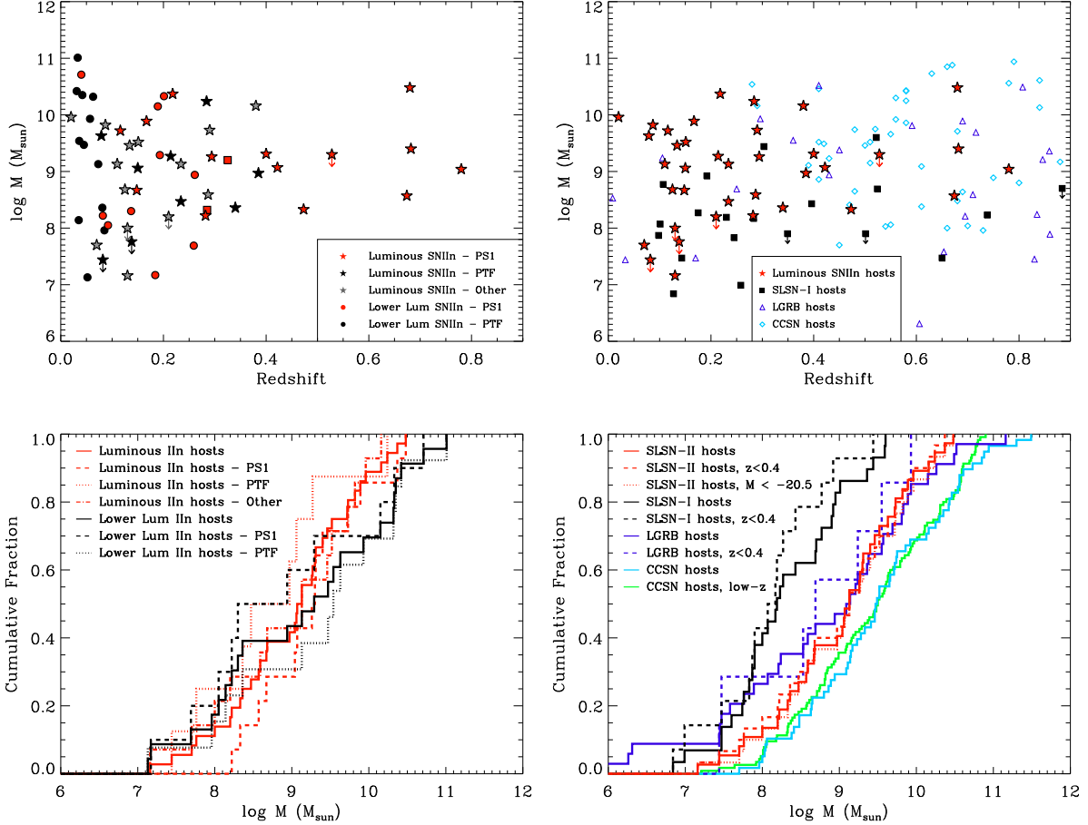
Figure 7.5.—: Same as Figure 7.3, but for host galaxy stellar masses. Symbols and colors have the same meaning as in Figure 7.2. Left: The host galaxies of luminous and standard luminosity Type IIIn SN both span approximately 4 orders of magnitudes 10^7 M_{\odot} < M_{\text{gal}} < 10^{11} M_{\odot} , and have similar median values of \langle M_{\text{gal}} \rangle \sim \times 10^9 M_{\odot} . Right: Luminous Type IIIn SN host galaxies are robustly distinguished from the the host galaxies of SLSN-I.
