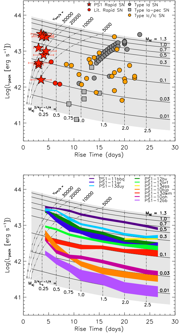
Figure 3.20.—: Physical constraints for ^{56}\text{Ni} powered explosions. Top Panel: We map the physical parameters M_{\text{Ni}} and M_{\text{ej}}^{3/4} E_{\text{K}}^{-1/4} onto the observable parameters of peak luminosity and rise time. On this we plot the gold/silver transients (red stars) and objects from the literature that are powered by radioactive decay (type Ia - grey circles; type Ib/Ic - orange circles; type Ia-pec - grey squares; rapid events - red circles). The curved lines represent locations where M_{\text{Ni}} = M_{\text{ej}} for a given ejecta velocity. Any object above and to the left of a given line is unphysical for that velocity. Bottom Panel: Colored regions represent the upper limit on the amount of ^{56}\text{Ni} which could power a second peak (such as that observed in SN 1993J) in the light curves of our objects.
