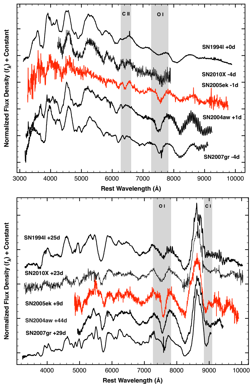
Figure 2.9.—: Comparison of SN 2005ek (red) and other well-studied SN Ic (black; SN 1994I, SN 2004aw, SN 2007gr, and SN 2010X). Strong similarities are seen. top : Near maximum light. The regions around C II \lambda 6582 and O I \lambda 7774 are shaded. bottom : Transitional spectra. The region around O I \lambda 7774 and C I \lambda 9095 are shaded.
