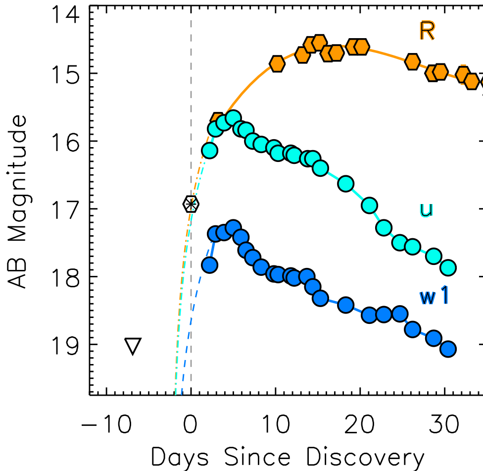
Figure 4.5.—: Characterization of the epoch of first light. Shown are the R-band (orange), u-band (cyan), and w1-band (blue) light curves, shifted to the AB system in the same manner as for Figure 4.2 (see Section 4.2.1). The rapid rise observed in the u- and w1-band light curves puts a tight constraint on the epoch of first light. Dashed colored lines are power law fits of the form t^{1.5} to the rising phase of each band, all of which imply an epoch of first light 2 days prior to first detection. The unfiltered discovery and pre-explosion limit are shown as a hexagon with an asterisk and an open triangle, respectively.
