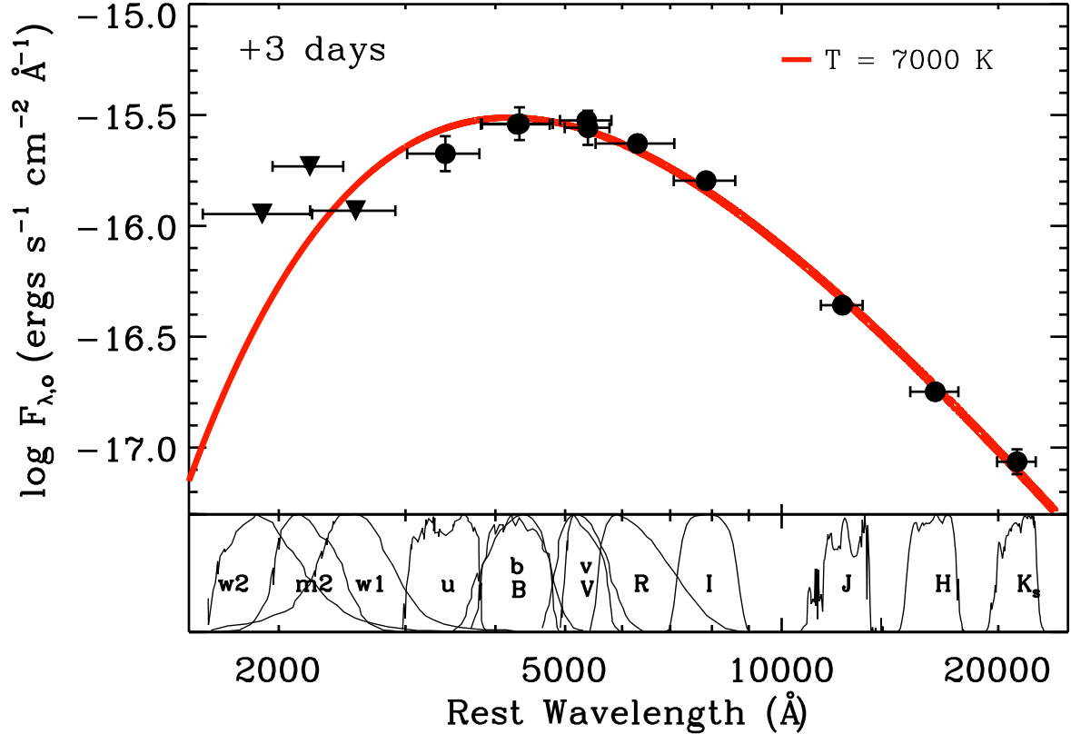
Figure 2.7.—: UV through IR spectral energy distribution of SN 2005ek at three days post-maximum. Upper limits are indicated as triangles and bandpass shapes are shown in the lower panel. The best-fitting 7000 K blackbody is shown as a red line.
