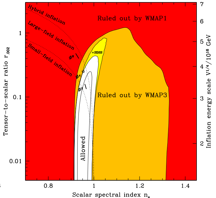
FIG. 19: 95% constraints in the (n_s, r_{0.002}) plane for 7-parameter tensor models (the vanilla parameters plus r ). The large shaded regions are ruled out by WMAP1 (red/dark grey) and WMAP3 (orange/grey). The yellow/light grey region is ruled out when adding SDSS LRG information, pushing the upper limit on r_{0.002} down by a factor of two to r_{0.002} < 0.33 (95%). The solid black curve without shading shows the 68% limit. The two dotted lines delimit the three classes of inflation models known as small-field, large-field and hybrid models. Some single-field inflation models make highly specific predictions in this plane as indicated. From top to bottom, the figure shows the predictions for V(\phi) \propto \phi^6 (line segment; ruled out by CMB alone), V(\phi) \propto \phi^4 (star; a textbook inflation model; on verge of exclusion) and V(\phi) \propto \phi^2 (line segment; the eternal stochastic inflation model; still allowed). These predictions assume that the number of e-foldings between horizon exit of the observed fluctuations and the end of inflation is 64 for the \phi^4 model and between 50 and 60 for the others as per [150].
