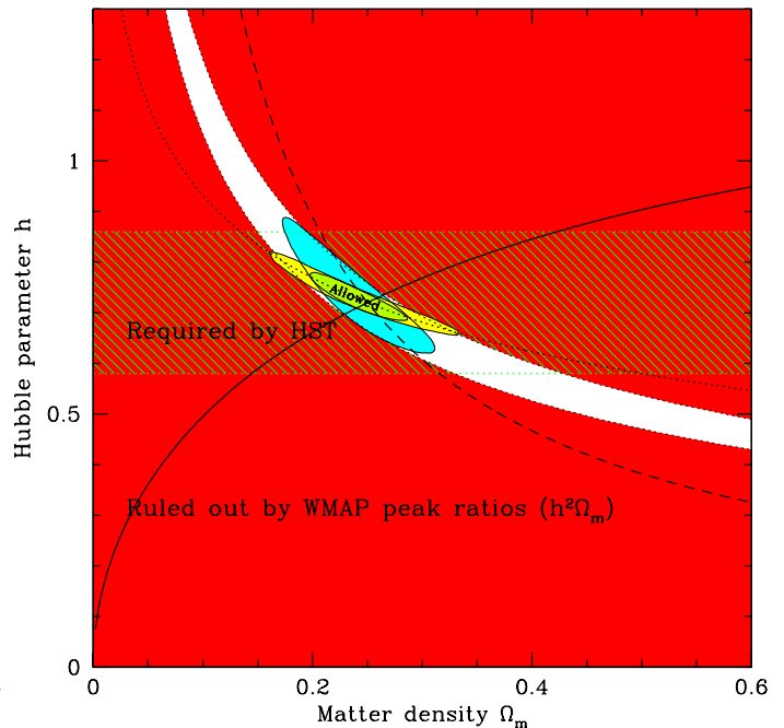
FIG. 14: Illustration of the physics underlying the previous figure. Using only WMAP CMB peak height ratios constrains (\omega_m, \omega_b, n_s) independently of A_s, \tau , curvature and late-time dark energy properties. This excludes all but the white band \omega_m \equiv h^2\Omega_m = 0.127 \pm 0.017 ( 2\sigma ). If we assume \Omega_{\text{tot}} = 1 and vanilla dark energy, we can supplement this with independent “standard ruler” information from either WMAP CMB (thin yellow/light grey ellipse) giving \Omega_m = 0.239 \pm 0.034 ( 1\sigma ), or SDSS galaxies (thicker blue/grey ellipse) giving \Omega_m = 0.239 \pm 0.027 ( 1\sigma ). These two rulers are not only beautifully consistent, but also complementary, with the joint constraints (small ellipse marked “allowed”) being tighter than those from using either separately, giving \Omega_m = 0.238 \pm 0.017 ( 1\sigma ). The plotted 2-dimensional constraints are all 2\sigma . The three black curves correspond to constant “horizontal” observables: constant angular scales for the acoustic peaks in the CMB power (dotted, h \propto \Omega_m^{-0.3} ), for the acoustic peaks in the galaxy power (solid, h \propto \Omega_m^{0.37} ) and for the turnover in the galaxy power spectrum (dashed, h \propto \Omega_m^{-0.93} ). This illustrates why the galaxy acoustic scale is even more helpful than that of the CMB for measuring \Omega_m : although it is currently less accurately measured, its degeneracy direction is more perpendicular to the CMB peak ratio measurement of h^2\Omega_m .
