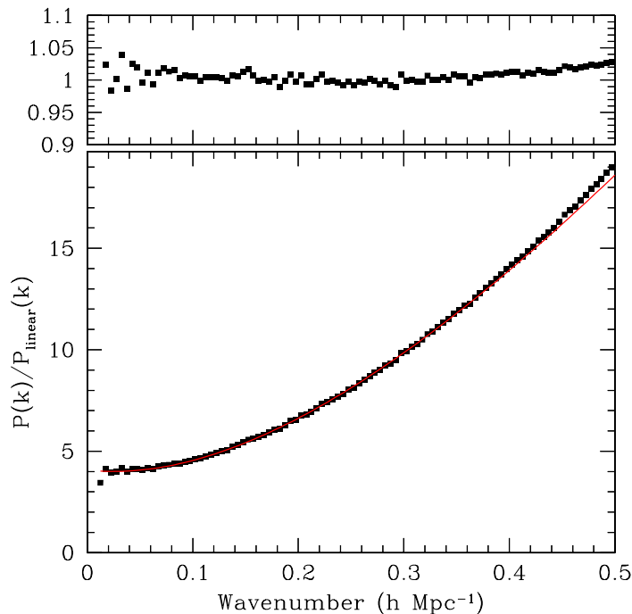
FIG. 10: The points in the bottom panel show the ratio of the real-space power spectrum from 51 averaged n -body simulations (see text) to the linear power spectrum dewiggled with k_* = 0.1h/\text{Mpc} . Here LRGs were operationally defined as halos with mass exceeding 8 \times 10^{12} M_\odot , corresponding to at least ten simulation particles. The solid curve shows the prediction from equation (4) with b = 2.02 , Q_{\text{nl}} = 27 , seen to be an excellent fit for k \lesssim 0.4h/\text{Mpc} . The top panel shows the ratio of the simulation result to this fit. Although the simulation specifications and the LRG identification prescription can clearly be improved, they constitute the first and only that we tried, and were in no way adjusted to try to fit our Q_{\text{nl}} = 30 \pm 4 measurement from Table 2. This agreement suggests that our use of equations (4) and (5) to model nonlinearities is reasonable and that our measured Q_{\text{nl}} -value is plausible.
