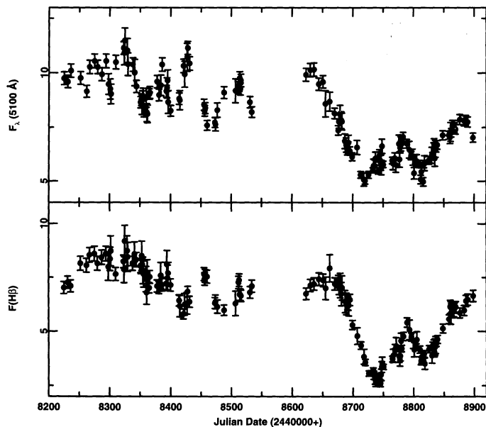
FIG. 1.—The continuum fluxes at 5100 \text{\AA} (top panel) and \text{H}\beta emission-line fluxes (bottom panel) for NGC 5548, as given in Table 5, from 1990 December to 1992 October. Fluxes are in the rest frame of NGC 5548, and are in units of 10^{-15} ergs \text{s}^{-1} \text{cm}^{-2} \text{\AA}^{-1} for the continuum and 10^{-13} ergs \text{s}^{-1} \text{cm}^{-2} for the line.
