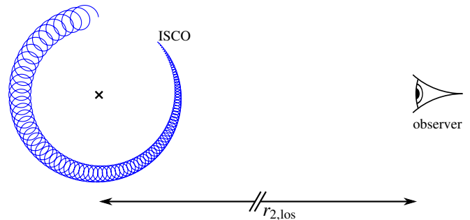
Figure 1. A schematic illustration of the triple systems under consideration (not to scale). The blue curve represents the trajectory of one component of the inspiraling “inner binary”. The inner binary separation a_1 shrinks because of gravitational wave emission, while its center of mass orbits around the triple system’s center of mass (marked with a cross) forming an “outer binary” with separation a_2 \gg a_1 . The blue curve starts when the inner binary’s gravitational wave (GW) frequency enters the detector’s sensitive range, and ends when the inner binary reaches the innermost stable circular orbit (ISCO) and coalesces. Depending on the three masses and a_2 , the inner binary may complete thousands of inner orbits and multiple revolutions around the triple’s center of mass while in the LIGO/VIRGO band, whereas for others it completes only a small fraction of an outer orbit (see Equation 4).
