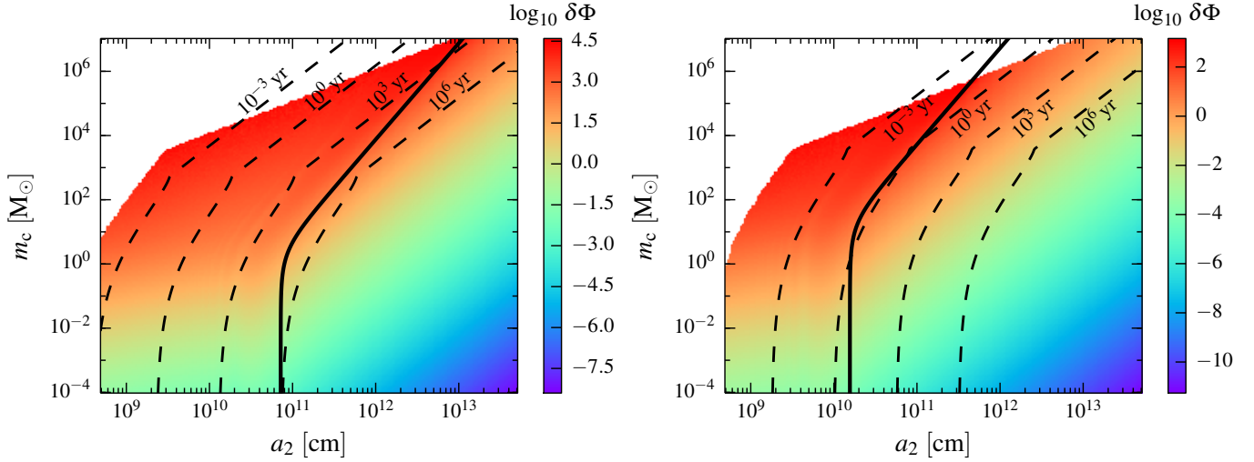
Figure 3. The total Doppler phase shift of the GW signal compared to a reference waveform, from a merging NS-NS binary ( left panel ) and a BH-BH binary ( right panel ) due to a perturber, while the signal is in the LIGO/VIRGO frequency band; \log_{10} \delta\Phi is shown as a function of the perturber’s distance and mass. For systems along the thick solid line, the outer binary has completed one radian of its orbit while the system is in the LIGO band (left of the curve means larger fraction of the orbit). The triple system is unstable in the white region on the top left due to either Newtonian dynamical reasons or the outer separation is smaller than the ISCO; the dashed lines represent the time that the system could have been dynamically stable (i.e. has existed no longer than the amount of time shown on the line). The signal may be detectable if \log_{10} \delta\Phi \gtrsim 0 and the source is within the LIGO horizon. The only LIGO-specific information that enters into this figure is f_{\min} = 10\text{Hz} as it determined the signal’s duration, the phase shift is otherwise independent of detector properties and the source’s distance.
