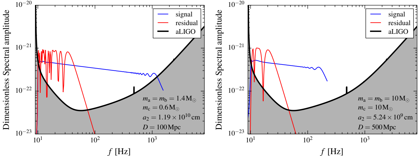
Figure 2. The dimensionless gravitational wave spectral amplitude (blue curve) and root mean square (rms) spectral noise amplitude per logarithmic frequency bin of Advanced LIGO (black curve) from a merging binary system of ( left panel ) two 1.4M_{\odot} neutron stars (NSs) with a 0.6M_{\odot} white dwarf companion on a circular orbit at a separation 1.185 \times 10^{10} cm located at a distance of 100 Mpc from the Earth; ( right panel ) two 10M_{\odot} black holes (BHs) with another 10M_{\odot} BH companion on a circular orbit at a separation 5.244 \times 10^9 cm located at a distance of 500 Mpc from the Earth. The red curves show the spectral density of the residual between the signal and a reference signal of a merging binary with no triple companion. The signal progresses in time from left to right; the line ends when the (inner) binary reaches the innermost stable circular orbit (ISCO). The coalescence and ringdown phases are not shown.
