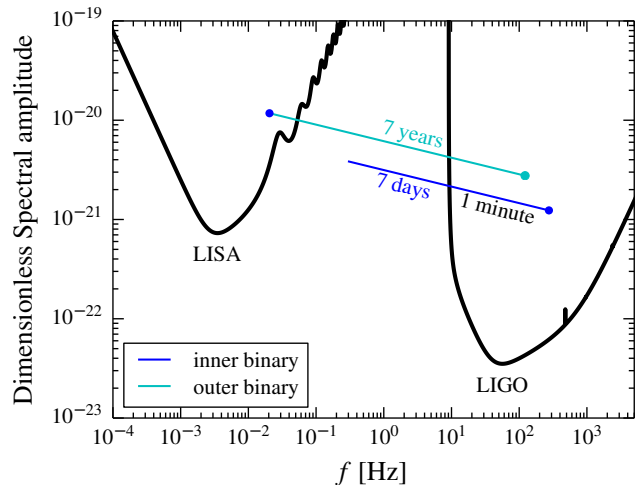
Figure 5. The dimensionless spectral amplitude due to a triple system comprised of a circular inner binary of two 8M_{\odot} BHs and a 20M_{\odot} companion BH, at a distance of 100 Mpc. The inner binary is in the LIGO band for 55 sec, during which the triple companion induces a Doppler shift \delta\Phi of 5.8 rad. Stability analysis shows that such a circular system must have formed in at most 6.9 days before the inner binary signal was detected with LIGO. The GW frequency of the outer binary is in the LISA band during the LIGO detection. Following the inner binary merger, the outer binary GW frequency leaves the LISA band and 6.7 years later enters the LIGO band. The filled blue circles represent the ISCO of the inner binary, the cyan circle represents the ISCO of the outer binary (the ringdown is not shown for either binary).
