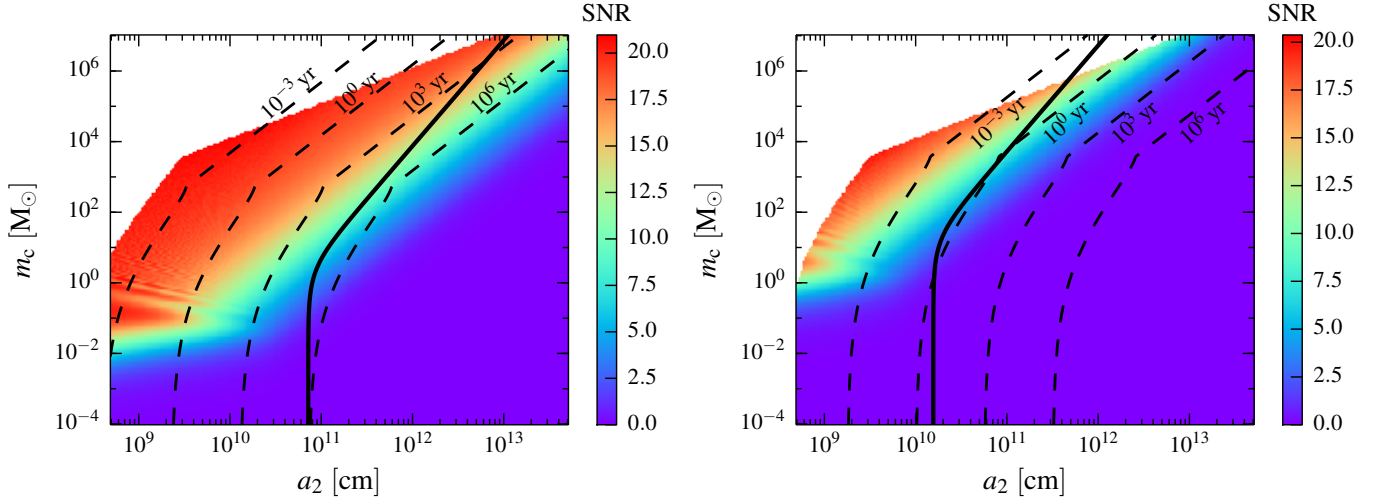
Figure 4. Similar to Figure 3 but now showing the signal-to-noise ratio of the residual between the signal and the reference waveform. The Advanced LIGO sensitivity curve is used, and the NS-NS binary ( left panel ) is put at 100Mpc from the Earth, while the BH-BH binary ( right panel ) is put at a distance of 500Mpc.
