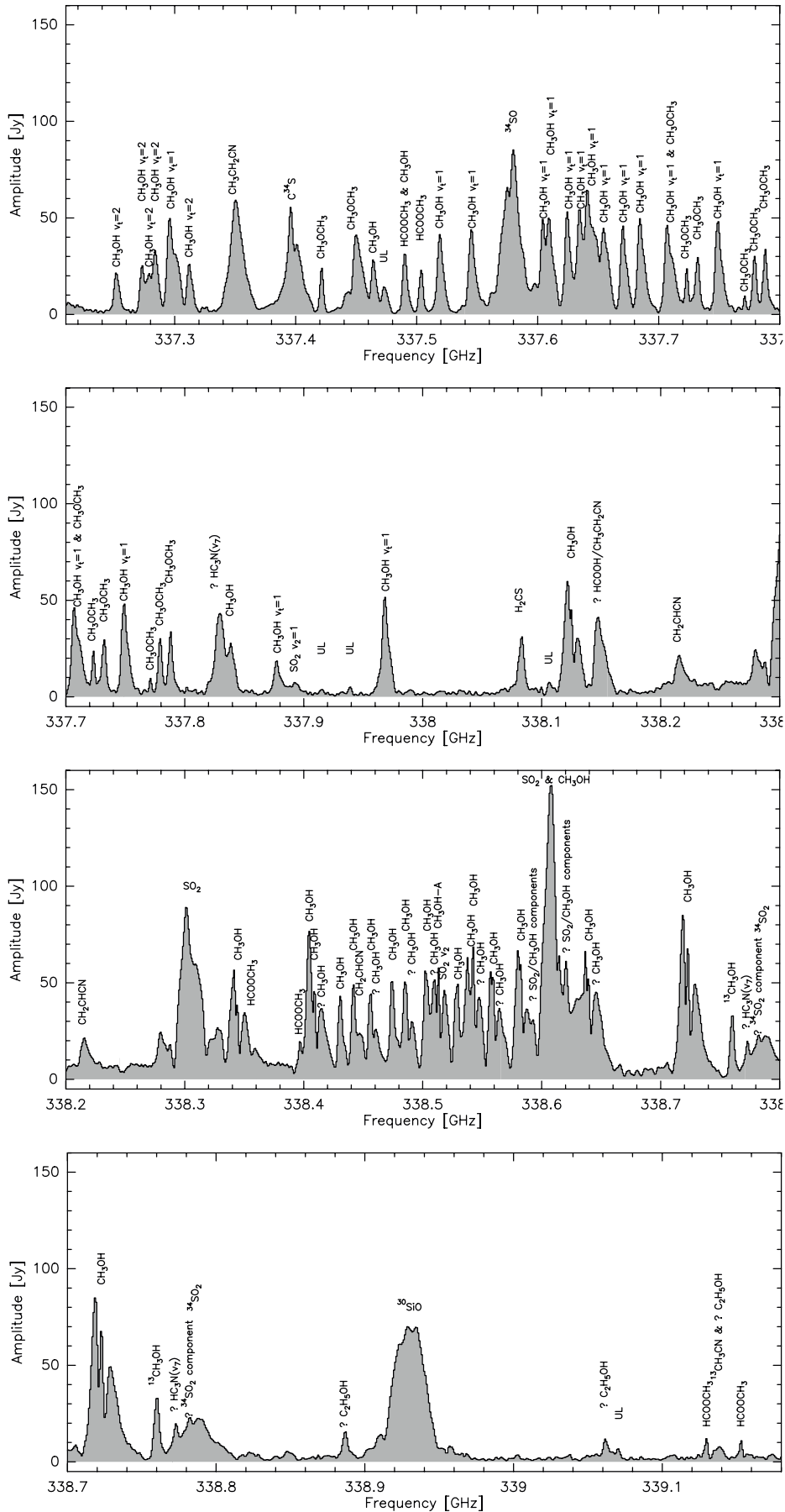
Fig. 4.—Vector-averaged lower sideband spectra (ZOOM) in the u - v domain on a short baseline of \sim 21 m. The spectral resolution is 0.7 \text{ km s}^{-1} . UL marks unidentified lines, and question marks indicate only tentatively identified lines.
