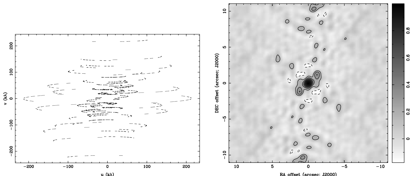
Fig. 2.—Left: Resulting u - v coverage from the two observed tracks. Right: Image of the dirty beam. The contour levels are -0.125 (dashed line) and 0.125-1 in 0.125 level steps (solid lines).
