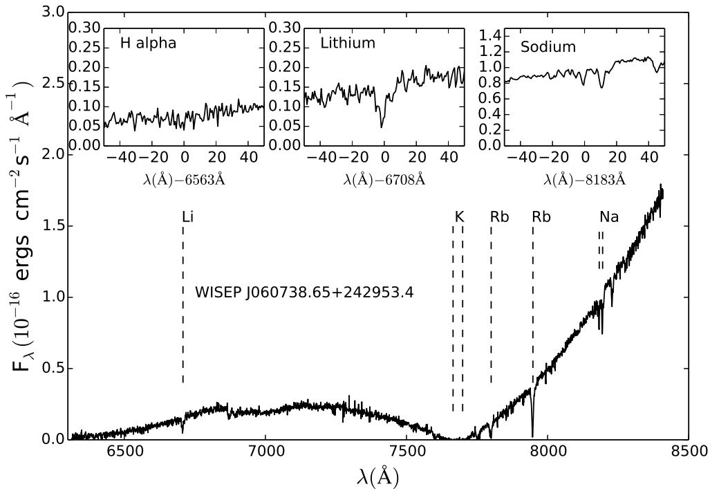
Figure 1. Optical spectrum of W0607+24. We detect lithium absorption but no H \alpha emission or absorption.
