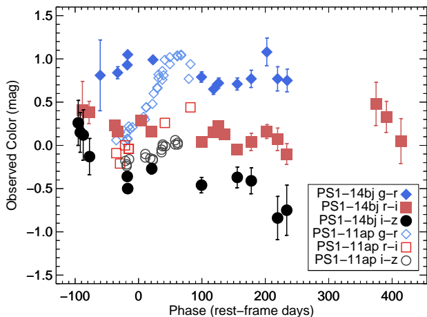
Figure 5. Color evolution of PS1-14bj (filled symbols). The open symbols show the more typical H-poor SLSN PS1-11ap (McCrurn et al. 2014), which was at almost exactly the same redshift as PS1-14bj ( z = 0.524 ), facilitating comparison. PS1-14bj is significantly redder than PS1-11ap in its early phases, particularly seen in the observed g-r color. Also note the remarkably flat color evolution of PS1-14bj, with an overall trend towards bluer colors with time, particularly in i-z . In contrast, PS1-11ap (like most supernovae) turns redder with time.
