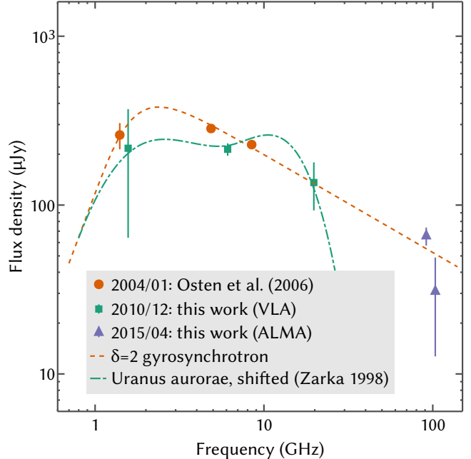
Figure 3. Non-simultaneous centimeter-to-millimeter spectrum of TVLM 513. The orange points show the data obtained quasi-simultaneously by Osten et al. (2006); green show the quasi-simultaneous VLA data described in Section 3.2; blue show the simultaneous ALMA data described in Section 3.1. The dashed lines show two representative spectral models described in Section 4.2; they disregard the long time baseline between the relevant VLA and ALMA observations and should not be used for quantitative analysis.
