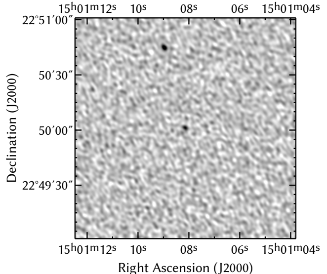
Figure 1. ALMA detection image of TVLM 513 . The effective frequency of the image is 97.48 GHz, the total bandwidth is 8 GHz, the grayscale runs from -20 \mu\text{Jy} (white) to 65 \mu\text{Jy} (black), and the image rms is \sim 8.4 \mu\text{Jy} . A source is detected at the expected position of TVLM 513 with a flux density of 55 \pm 12 \mu\text{Jy} , where the uncertainty in the flux density comes from least-squares fitting the pixel data. The synthesized beam is 3.1 \times 2.2 arcsec at a position angle of 44^\circ .
