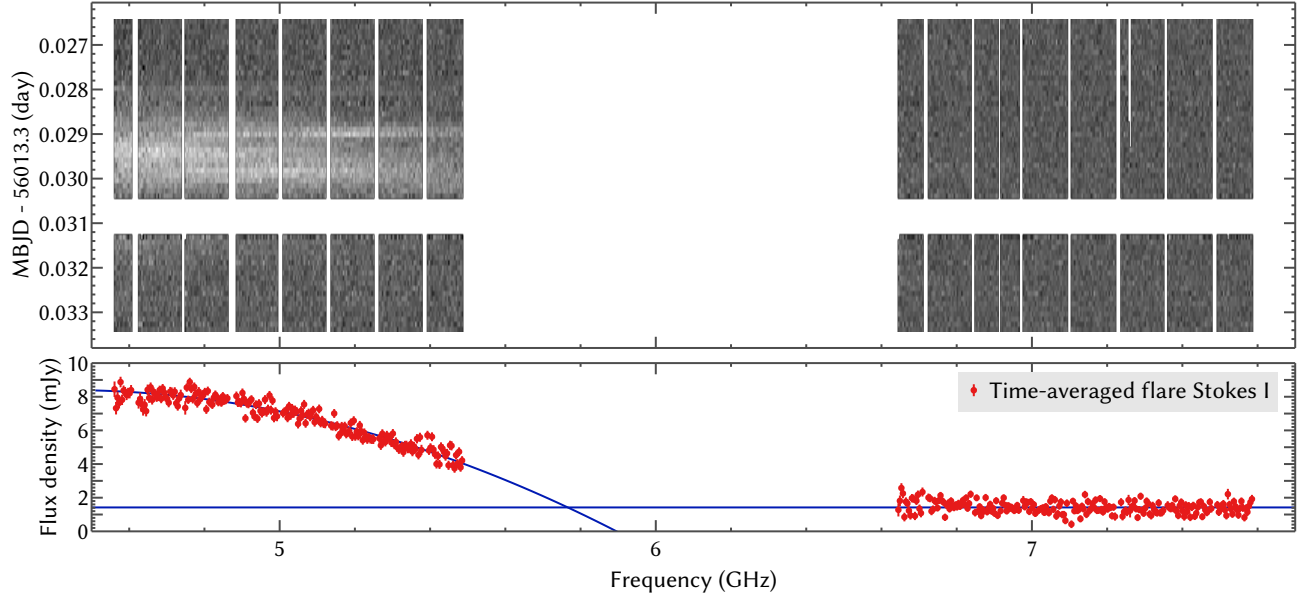
Figure 7. Upper panel: Stokes I dynamic spectrum of the bright radio flare seen in day 2 of Campaign 1. The measurements are made at a 10 s cadence and the grayscale runs linearly from -7.2 mJy (black) to 17.1 mJy (white). The large frequency gap in the data is due to the positioning of the VLA basebands; all others are due to RFI. The non-flaring variation has not been subtracted (Section 4.2). Lower panel: the flare spectrum averaged between 0.0286 < \text{MBJD} - 56013.3 < 0.0304 . The flare is absent from the 7.1 GHz frequency window. Also shown are parabolic (constant) fits to the spectrum in the lower (upper) frequency windows. These fits suggest that the flare cutoff frequency is \sim 5.8 GHz. The flare light curve is shown in Figure 8.
