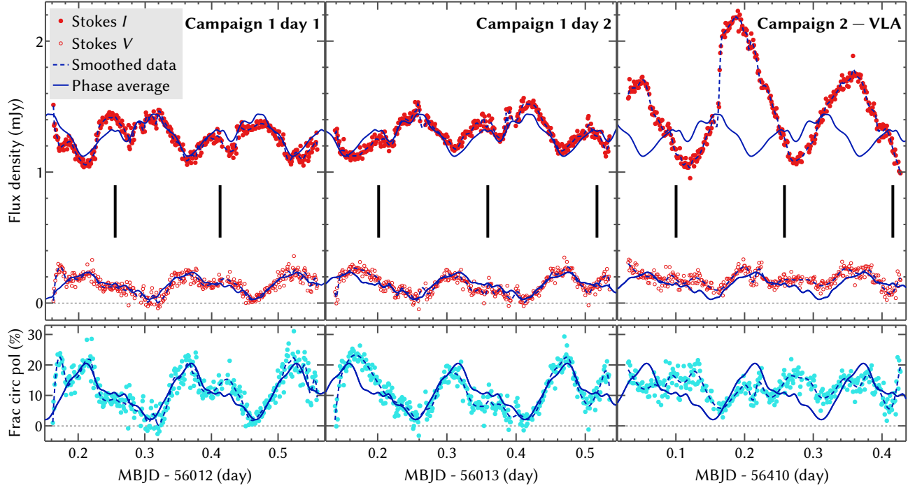
Figure 9. VLA light curves with 100% LCP flares removed. Stokes I , Stokes V , and f_c are shown. Vertical black lines indicate times of maximum flux in the primary MEarth periodic component. Dashed blue lines show smoothed spline fits to the data. Solid blue lines trace mean profiles of the Campaign 1 data after phasing to the primary MEarth periodicity (see Section 4.2). While the Campaign 2 Stokes I data disagree with the Campaign 1 mean phase profile, the Stokes V data show broadly similar structure.
