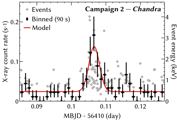
Figure 11. Zoom-in of the rapid X-ray flare. Along with the model as in Figure 10, individual events are shown with vertical positions indicating energy as shown on the right axis . Binned and model count rates are associated with the left axis . The binning interval is 90 s.
