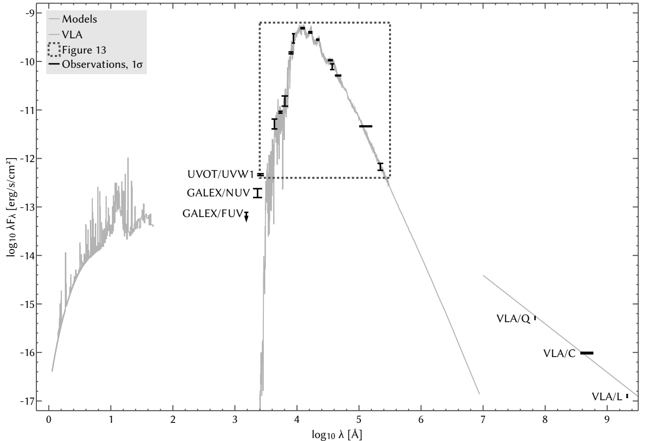
Figure 14. The ultra-wideband, non-simultaneous, blended SED of NLTT 33370 AB . The dashed box identifies the region shown in Figure 13, in which the enclosed observational data are identified. The short-wavelength model curve shows the best-fitting two-temperature APEC source model fit as described in Section 4.3; the observed X-ray data cannot be displayed in flux density units because the incident photon energies are only known in a probabilistic sense. The middle model curve is the best-fit BT-Settl model as described in Section 5.1. The long-wavelength model curve is a constant flux density of 1.3 mJy. Also shown are measurements from GALEX (Martin et al. 2005), McLean et al. (2011, “VLA/L”), and this work (see Section 5.1 for details).
