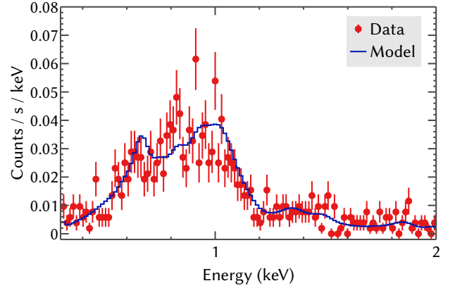
Figure 12. Chandra X-ray spectrum and a fitted two-temperature solar abundance APEC model. The temperatures of the two components are kT = 0.27(2) keV and 1.20(6) keV.
