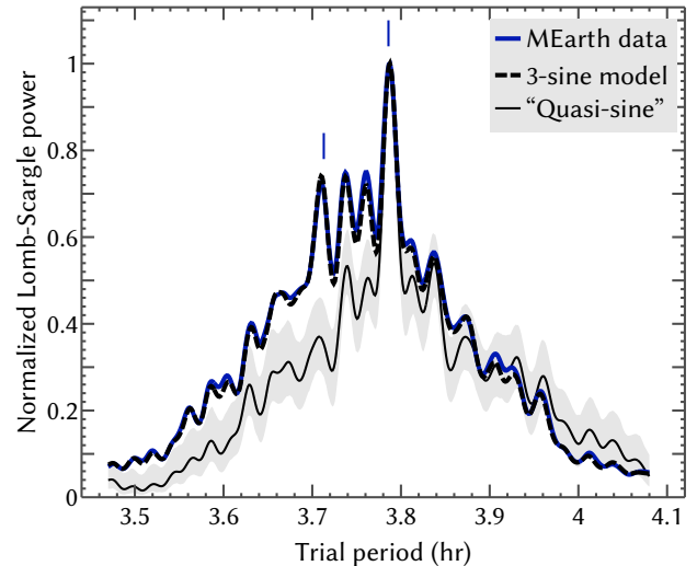
Figure 6. Lomb-Scargle periodograms for the Campaign 1 MEarth data. The periodogram for the systematics-corrected data is shown in blue with the peak normalized to unity. The dashed black line shows the normalized periodogram for the 3-sine model, using the same sampling as the data; it is nearly identical to the data periodogram. The thin black line shows the periodogram for a single-sine fit; its gray envelope shows the 90% credible region for a “quasi-sine” model with a single periodicity, but random amplitude and phase perturbations that vary with 2–400 hr autocorrelation timescales. See Section 4.1 for details. This model does not reproduce the observed periodogram structure. The short, vertical blue lines indicate the primary and secondary periods determined for the 3-sine model.
