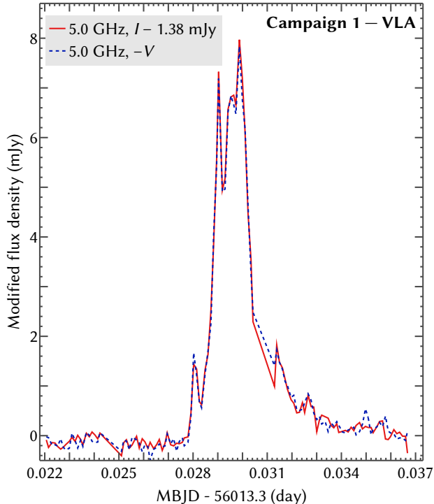
Figure 8. Light curve of the radio flare shown in Figure 7 averaging across the lower (5.0 GHz) baseband. Both Stokes I and V are shown. Because the flare is essentially 100% LCP, -V is plotted to maintain positivity. The nonflaring, unpolarized emission has been removed by subtracting median (I + V) = 1.38 mJy from the Stokes I data. Errors are \sim 0.1 mJy.
