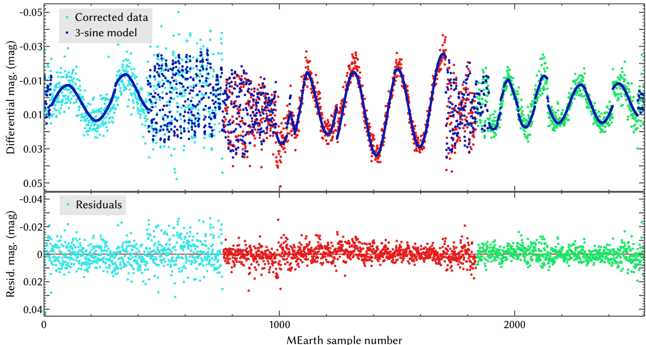
Figure 5. Data, model, and residuals for the complete MEarth dataset. For clarity, the abscissa is a monotonically-increasing sample number rather than, e.g., the observation time; the data span 3.4 yr. Data and residuals from Campaigns 0, 1, and 2 are shown in light blue, red, and green, respectively. The model is shown in dark blue. The “intensive” observing runs are apparent as segments of smoothly-varying data. The data shown here have been corrected for MEarth photometric systematics as described in Sections 3.1 and 4.1.
