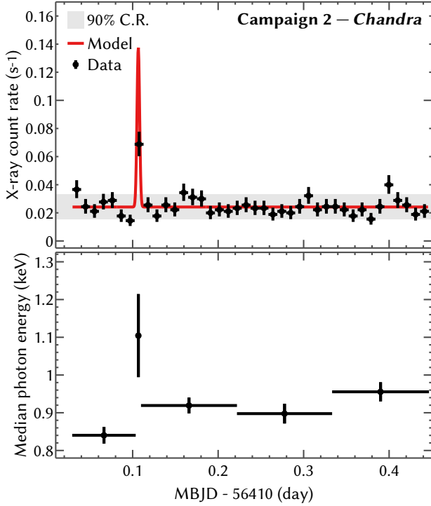
Figure 10. Chandra observations in Campaign 2. Black points in the upper panel show the count rate in uniform 15-min bins. The red line shows an analytic model fit to the unbinned data (see Section 4.3). The gray band shows the 90% confidence region for samples of the quasi-quiet emission; most of the apparent variability is not significant. The lower panel shows the change in the X-ray spectrum as quantified in the median photon energy (Hong et al. 2004). The increase in the hardness of the quasi-quiet emission may be a precursor to the long-duration flare detected by Swift .
