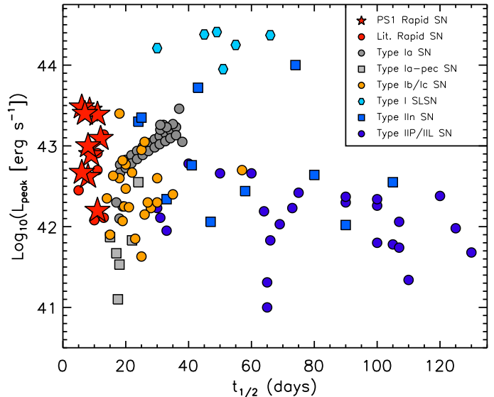
FIG. 7.— The phase space of SN: peak luminosity versus rest-frame time above half-maximum for a variety SN. The PS1-MDS transients described in this paper are shown as red stars. They span an order of magnitude in peak luminosity and significantly increase the number of known transients with short characteristic times. Other events from the literature are shown as colored circles/squares: type Ia SN (Nugent et al. 2002; Taubenberger et al. 2008; Scalzo et al. 2012), type Ia-x & “calcium-rich” Ia (Foley et al. 2013; Kasliwal et al. 2012; Perets et al. 2010), type Ib/Ic SN (Drout et al. 2011; Valenti et al. 2008; Campana et al. 2006; Taubenberger et al. 2006; Bersten et al. 2012; Olivares et al. 2012; Cobb et al. 2010; Valenti et al. 2012), type IIP/IIL (Arcavi et al. 2012; Hamuy 2003; Andrews et al. 2011; Botticella et al. 2009), type IIn (Kiewe et al. 2012; Margutti et al. 2014), type I SLSN (Quimby et al. 2011; Chomiuk et al. 2011; Lunnan et al. 2013), and other rapidly-evolving events (red; Drout et al. 2013; Kasliwal et al. 2010; Poznanski et al. 2010; Ofek et al. 2010; Matheson et al. 2000).
