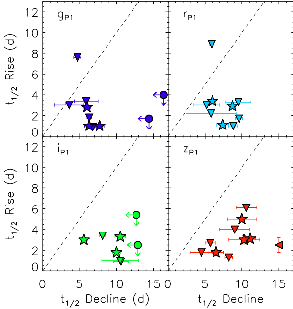
FIG. 8.— t_{1/2, \text{rise}} versus t_{1/2, \text{decline}} for the gold and silver transients in four photometric bands ( \text{grizP}_1 ). Stars represent objects with measured rise and decline timescales, triangles represent objects with an upper limit in one of the two timescales, and circles with arrows represent objects with upper limits for both timescales. In general, the PS1-MDS rapidly-evolving transients rise significantly faster than they decline.
