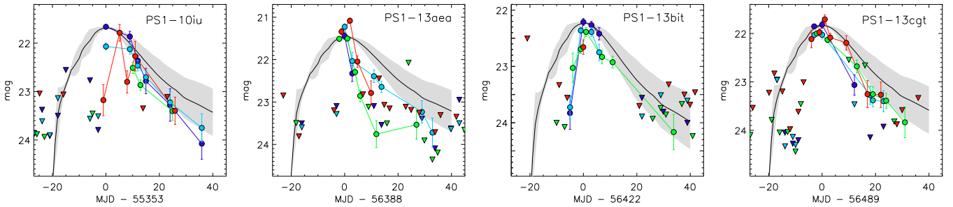
FIG. 3.— PS1 apparent magnitude, observer-frame, light curves for our bronze (non-spectroscopic) sample. Symbols have the same meaning as Figure 1.
