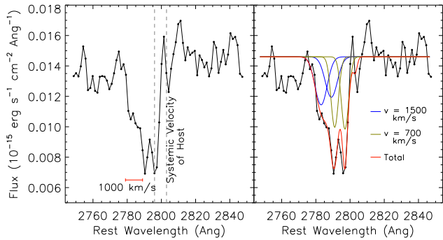
FIG. 14.— Mg II absorption in the spectrum of PS1-12bv. Left: Vertical lines mark the systemic velocities of the host galaxy as measured from [OII] \lambda 3727 and H\beta in emission. The red line signifies the extent of the resolved blue “shelf”, which may be due to absorption in the CSM surrounding the progenitor. Right: An example multiple component fit to the absorption feature. The green (blue) components are blue shifted \sim 700 km s^{-1} ( 1500 km s^{-1} ) with respect to the host galaxy and have a FWHM of 550 km s^{-1} ( 900 km s^{-1} ). The galaxy [OII] \lambda 3727 feature has a FWHM of 300 km s^{-1} .
