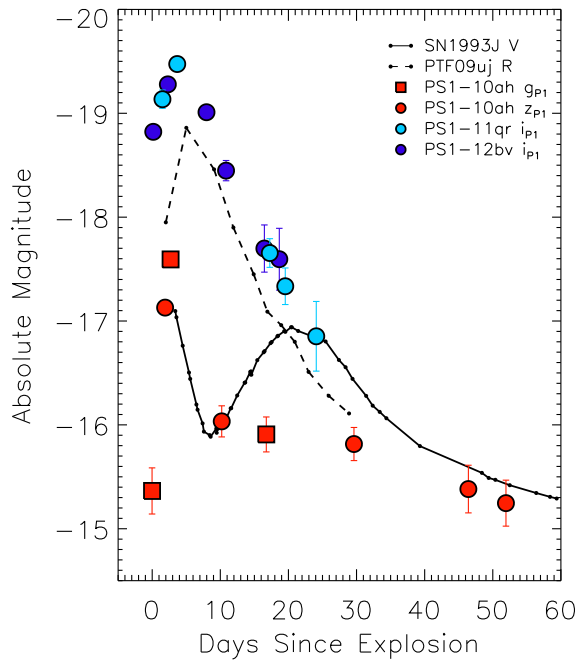
FIG. 21.— A comparison of the light curves of several gold transients to events from the literature thought to be powered by varieties of shock breakout/cooling envelope emission. PS1-10ah shows a similar initial decline to the type IIb SN 1993J, but lacks a later peak powered by radioactive decay. PS1-11qr, PS1-12bv, and a number of the other luminous events are very similar to PTF09uj, which was hypothesized to be due to the shock breakout from an optically thick wind (Ofek et al. 2010).
