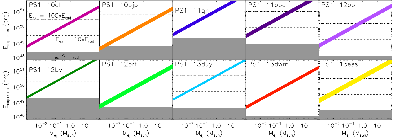
FIG. 23.— Values of M_{\text{ej}}E^{-1/2} derived for the gold/silver transients for the case of a shock breakout from a dense, optically thick, wind. The width of the colored region gives the error inferred for M_{\text{ej}}E^{-2} based on the errors for each of our observables. Grey shading represents an excluded region where the explosion energy is less than the observed radiated energy. Horizontal lines in each panel represent where E_{\text{explosion}} = 10 \times E_{\text{rad}} and 100 \times E_{\text{rad}} for each object.
