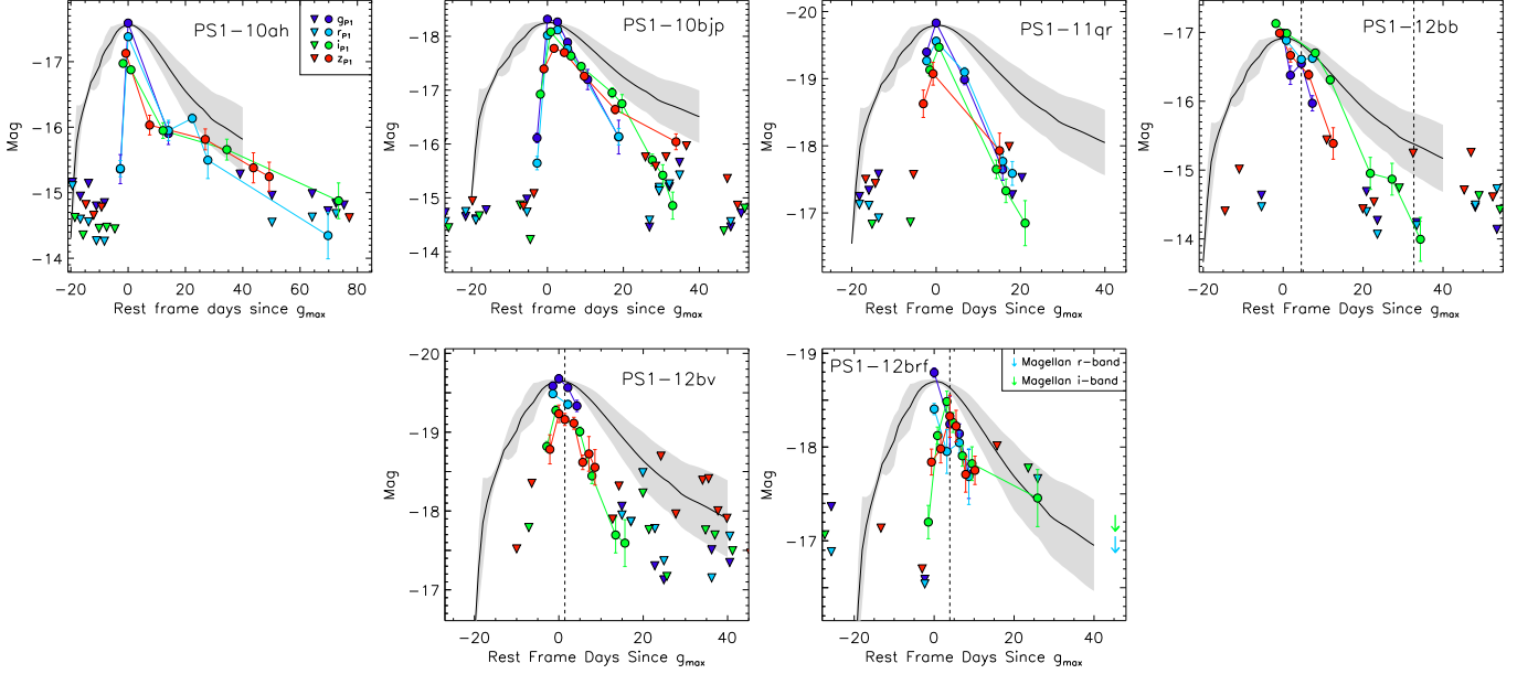
FIG. 1.— PS1 absolute magnitude, rest-frame, light curves for gold sample transients. Circles represent grizp_1 detections and triangles represent 3\sigma upper limits. Vertical dashed lines indicate epochs when spectroscopic observations were acquired. The grey shaded region is the R-band type Ibc template from Drout et al. (2011), normalized to the peak magnitude of the PS1-MDS transient.
