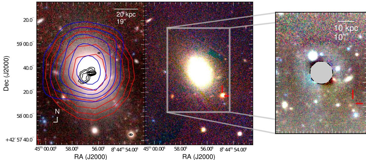
FIG. 1.— Multiwavelength observations of the field of PS1-12sk. Left: optical composite of g_{P1}r_{P1}z_{P1} pre-explosion PS1 images from December 2009 to May 2012, shown with log stretch. Contours from our 5.9 GHz JVLA observations are overlaid in black (beam FWHM \sim 3.5'' ), NVSS 1.4 GHz radio observations are overlaid in red (beam FWHM \sim 45'' ), and XMM-Newton X-ray observations are overlaid in blue (FWHM \sim 6'' ). The radio and X-ray emission is centered on CGCG 208-042, the brightest cluster galaxy. Middle: PS1 g_{P1}r_{P1}z_{P1} imaging of the environment near the peak of PS1-12sk (2012 March 13; MJD 55999), shown with linear stretch. The SN position is marked. Right: The deep composite with the model for the BCG subtracted (linear stretch; a 1 \times 1.33' field). The circular mask excludes the inner 7'' of the residual image for source detection.
