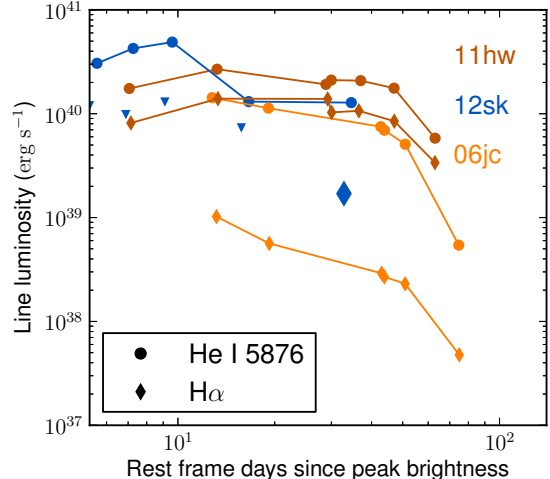
FIG. 9.— Comparison of intermediate-width line luminosity between PS1-12sk and the SNe Ibn 2006jc and 2011hw (Smith et al. 2012), \text{H}\alpha is only detected in the final spectrum (blue diamond) and limits (triangles) are plotted at earlier epochs.
