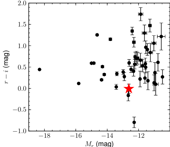
Fig. 7.— Color-magnitude diagram for sources in the field of CGC 208-042, assumed to be galaxies in the cluster RXC J0844.9+4258. The sources were detected on the BCG-subtracted PS1 images displayed in Figure 1. The source closest to PS1-12sk is marked with the red star. CGC 208-042, with M_r \sim -22.9 mag and (r - i) \sim 0.5 mag, is not shown.
