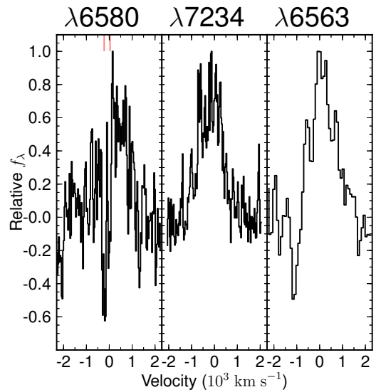
FIG. 6.— Left: moderate resolution MMT/BC spectroscopy of C II \lambda\lambda 6580, 7234 features in PS1-12sk from +8 d after z -band peak. The narrow absorption components corresponding to \lambda\lambda 6578, 6583 are marked with the red solid lines. Right: The H\alpha feature from the lower-resolution +35 days MMT spectrum. The velocity scale is relative to the He I narrow emission component, as in Figure 5.
