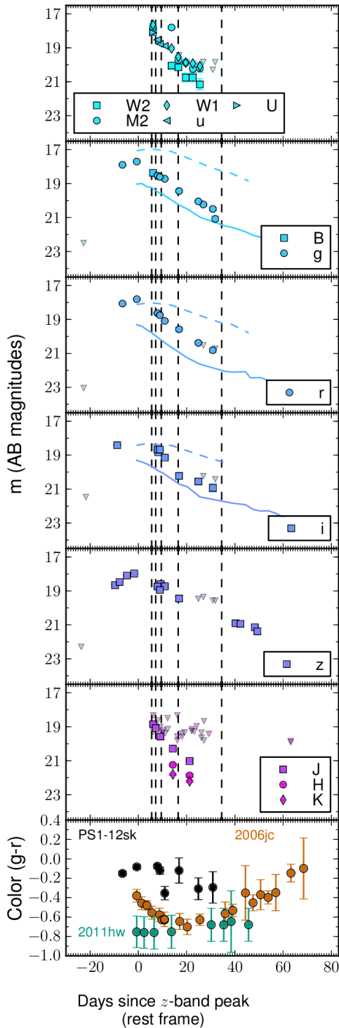
FIG. 3.— The multi-band light curve of PS1-12sk and 3\sigma upper limits (triangles). The thin lines are the BVRi light curves (AB magnitudes) of SN 2006jc (solid, Foley et al. 2007) and SN 2011hw (dashed, Smith et al. 2012), shifted temporally so the brightest/first observation corresponds to the epoch of z -band peak for PS1-12sk (MJD = 56006.1 \pm 0.3 ) and rescaled to z = 0.054 . The bottom panel shows the optical color (AB magnitudes), corrected for Galactic extinction, of PS1-12sk, SN 2006jc, and SN 2011hw (Smith et al. 2012). No extinction or K-corrections have been applied. The dashed vertical lines indicate the epochs of our optical spectroscopy.
