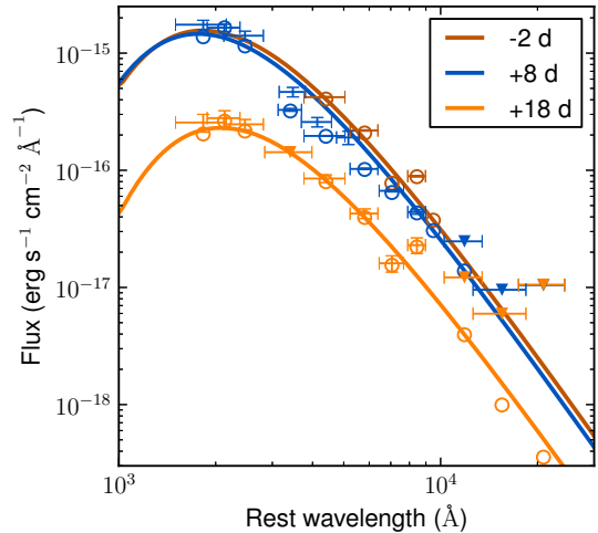
FIG. 4.— The SED of PS1-12sk from photometry at three epochs (MJD = [56005, 56015, 56025] \pm 1.5 ). The circles show the linearly-interpolated light curve value in each filter at each precise epoch, error bars show the flux and filter width for the measured NUV-NIR photometric points nearest to each epoch (only when within 1.5 days), and triangles show the nearest 3\sigma upper limit. The solid-lines show the blackbody fit to the interpolated photometry. The NIR observations do not suggest a significant infrared excess for PS1-12sk within a few weeks of peak brightness.
