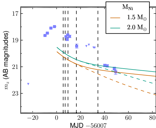
FIG. 8.— The z -band light curve of PS1-12sk alongside the nebular phase Type I SN light curve models described in Section 6.1. The models are shown with full (solid) and incomplete (dashed) gamma-ray trapping and assuming the explosion date is the same as the discovery date.
