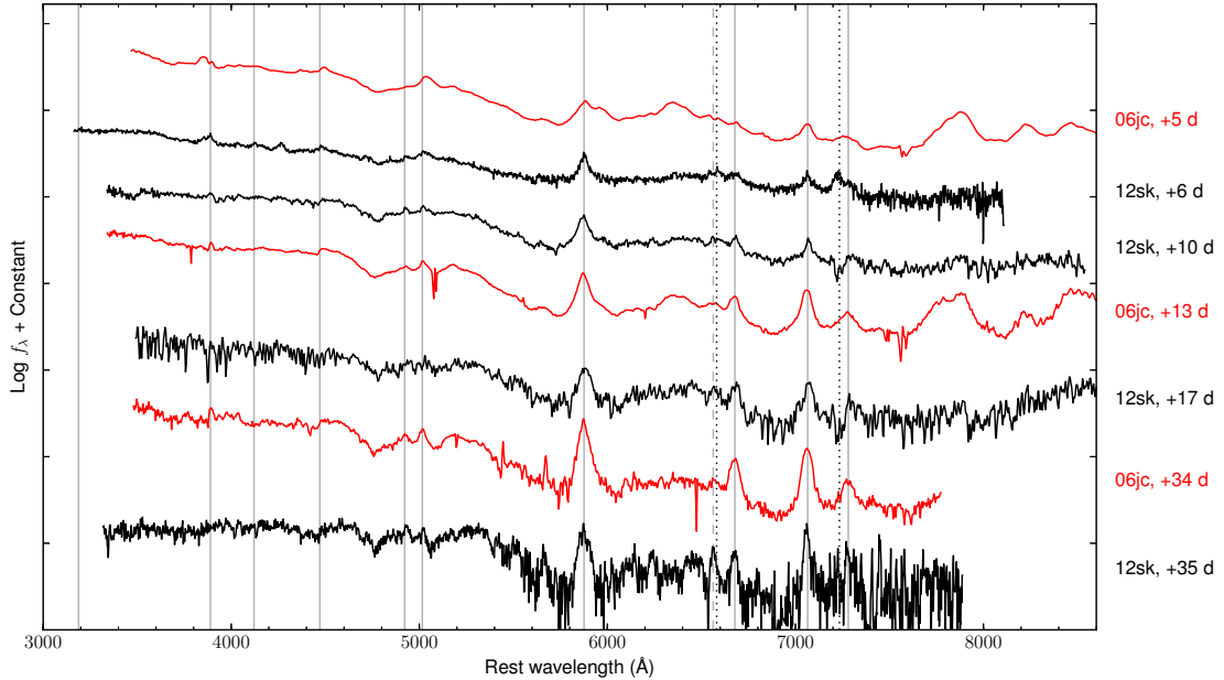
FIG. 2.— Low-resolution spectroscopic sequence of PS1-12sk, with time since z -band peak noted at right. See Table 2 for observing details. The moderate resolution MMT/BC spectrum is shown separately in Figure 5. The locations of the He I features \lambda\lambda 3188, 3889, 4121, 4471, 4922, 5016, 5876, 6678, 7065, 7281 Å are marked with solid lines; H\alpha with a dashed line; and C II \lambda\lambda 6580, 7234 with dotted lines. Spectra of SN 2006jc at representative epochs (Pastorello et al. 2008a) are shown in red.
