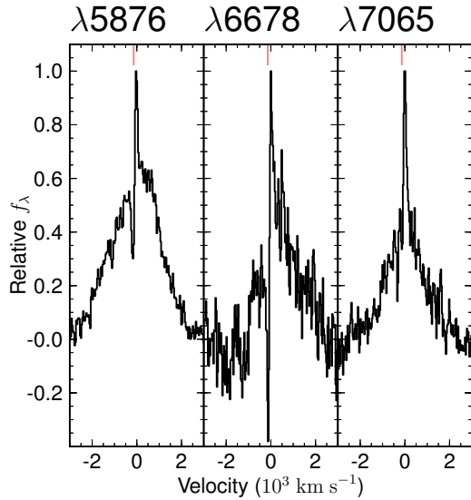
FIG. 5.— Moderate resolution MMT/BC spectroscopy of He I features in PS1-12sk from MJD 56014.2, +8 d after z -band peak. The velocity scale is centered on the narrow emission component of the P-Cygni profiles, blueshifted by 190 \text{ km s}^{-1} from the recession velocity of CGCG 208-042. The solid red line marks the center of the narrow absorption component, blueshifted by 140 \text{ km s}^{-1} relative to the emission.
