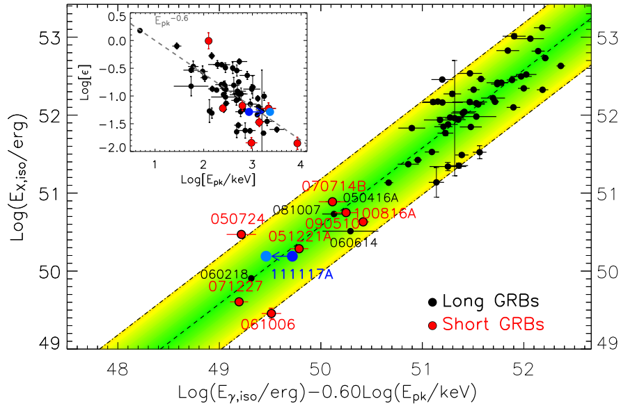
FIG. 7.— Three-parameter correlation involving the isotropic energy emitted in the X-ray afterglow ( E_{x,iso} ; rest-frame 0.3–30 keV), the isotropic \gamma -ray energy ( E_{\gamma,iso} ; rest-frame 1 – 10^4 keV), and the rest-frame spectral peak energy during the prompt phase ( E_{pk} ). The blue circles mark GRB 111117A using the range of E_{pk} \sim 850 –2300 keV (§2.1). The dot-dashed lines mark the 90% confidence area around the best-fit relation: E_{x,iso} \propto E_{\gamma,iso}^{1.00 \pm 0.06} E_{pk}^{-0.60 \pm 0.10} . The inset shows the evolution of \epsilon \equiv E_{x,iso}/E_{\gamma,iso} as a function of E_{pk} . Adapted from Margutti et al. (2012).
