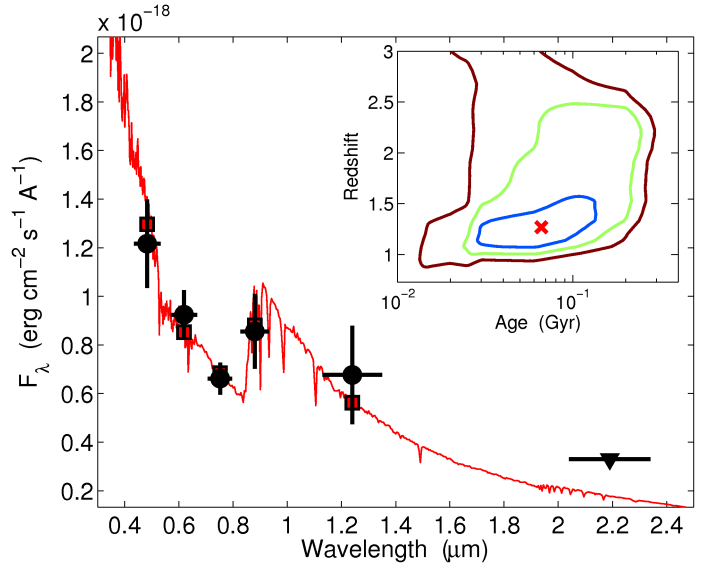
FIG. 4.— Optical and near-IR spectral energy distribution of the host galaxy of GRB 111117A (black), along with the Maraston (2005) evolutionary stellar population synthesis models. The best-fit model (red squares and line) has a photometric redshift of z \approx 1.3 and a stellar population age of \tau \approx 70 Myr (inset).
