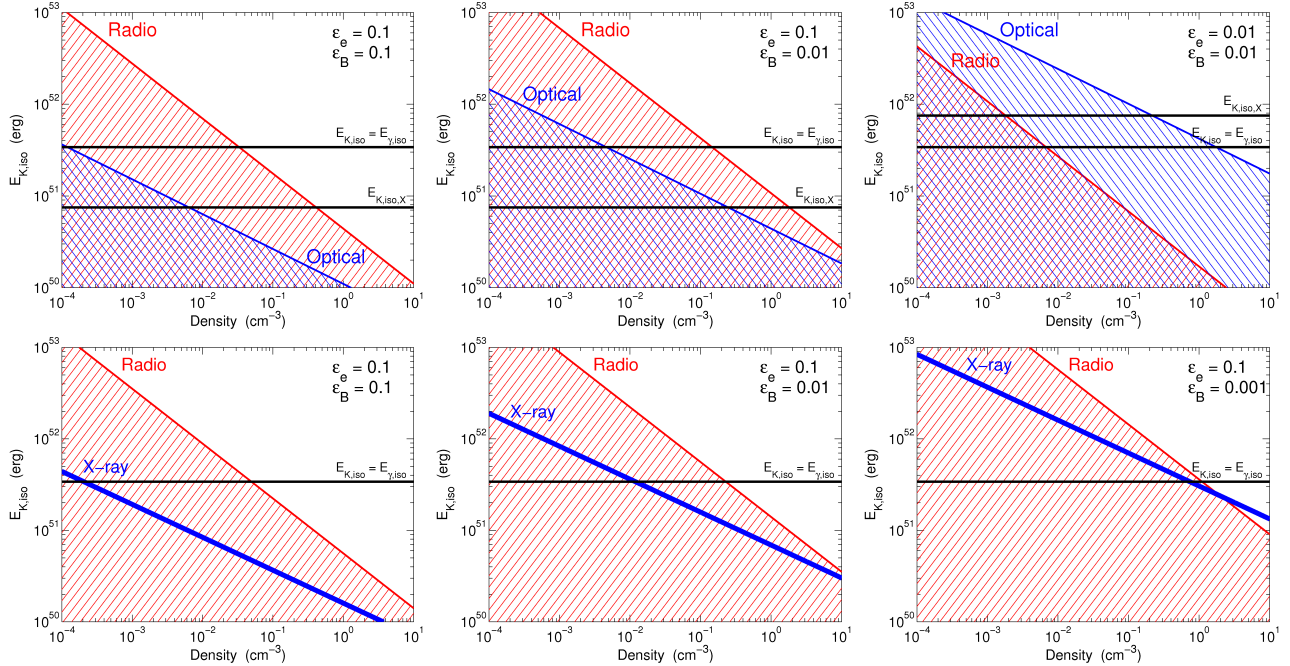
FIG. 9. — The phase-space of isotropic-equivalent blastwave kinetic energy and circumburst density delineated by the X-ray detection (thick line) and the optical and/or radio upper limits (hatched regions). The top row is for the case \nu_c < \nu_X , with the X-ray detection providing a measure of the E_{K,iso} (horizontal line). The bottom row is for the case \nu_c > \nu_X for which the optical limit is redundant with respect to the X-ray detection. Here the case of E_{K,iso} = E_{\gamma,iso} is marked by the horizontal black line. The panels are for different combinations of \epsilon_e and \epsilon_B .
