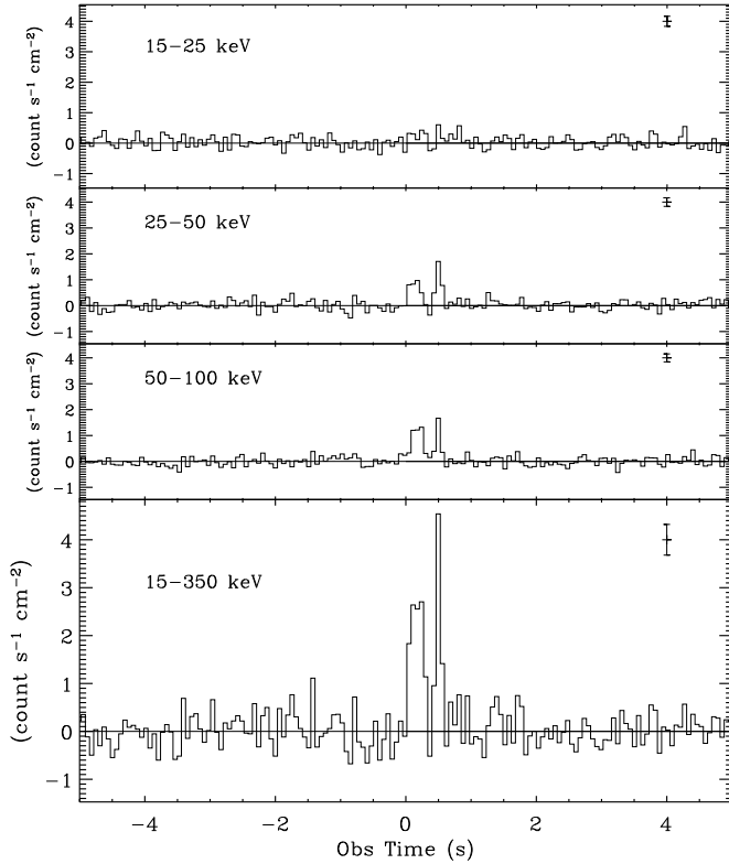
FIG. 1.— Swift /BAT mask weighted light-curve in different energy bands (binning time of 64 ms). The typical 1\sigma error-bar is shown in each panel.
