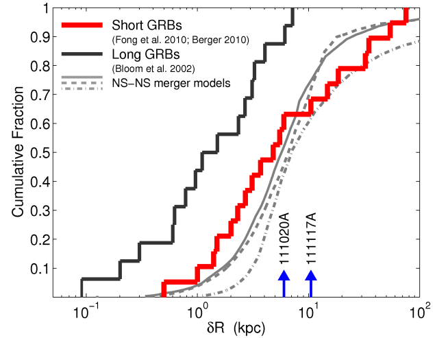
FIG. 5.— Cumulative distribution of projected physical offsets for short GRBs with sub-arcsecond positions (red; Fong et al. 2010; Berger 2010; Fong et al. 2012), including GRB 111117A, and for long GRBs (black; Bloom et al. 2002). Also shown are population synthesis model predictions for NS-NS binaries (Bloom et al. 1999; Fryer et al. 1999; Belczynski et al. 2006). Arrows mark the offsets of the two short GRBs localized by Chandra alone, GRB 111117A from this work and GRB 111020A from Fong et al. (2012). These offsets are somewhat larger than the median short GRB offset of about 5 kpc.
