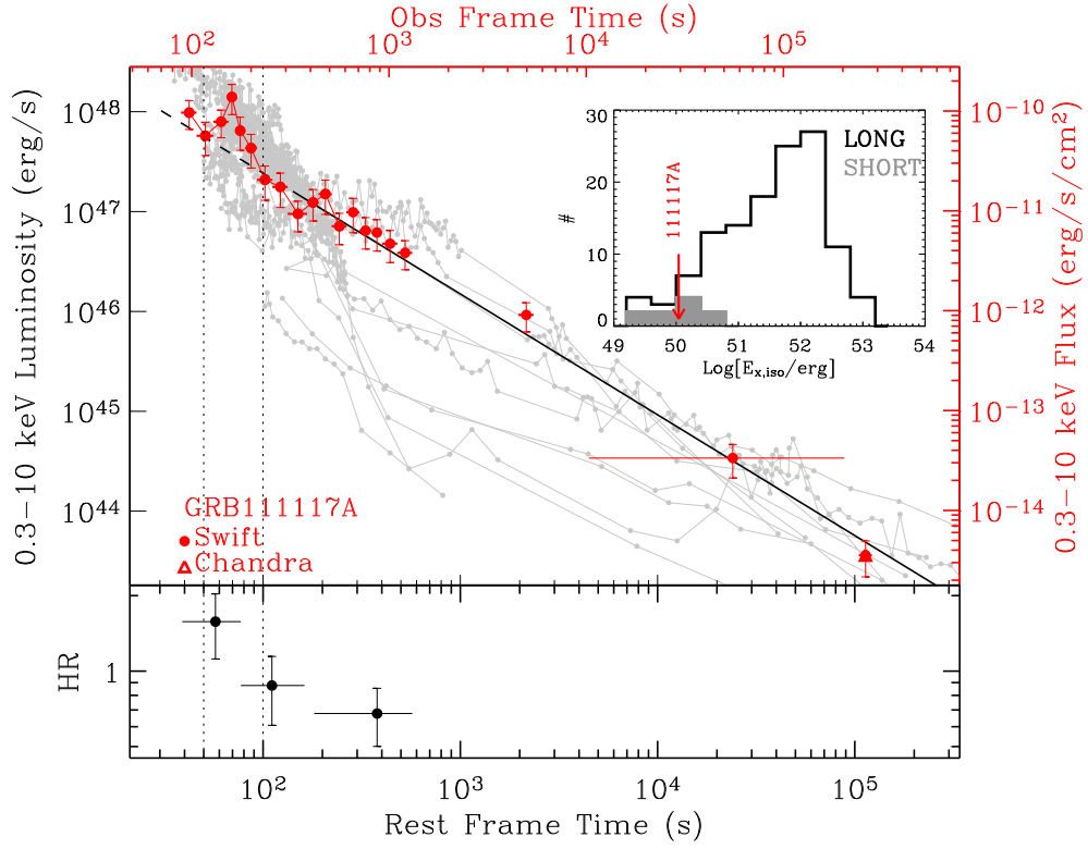
FIG. 6.— Upper panel : Unabsorbed 0.3–10 keV flux and luminosity light curve of GRB 111117A (red dots: Swift /XRT; red triangle: Chandra ) compared to 11 short GRBs detected by Swift for which a redshift measurement is available (grey lines). The best fit power-law model has \alpha_x = -1.21 \pm 0.05 (solid black line). An apparent flare is detected at \approx 80 –200 s (black dotted lines). The inset shows the distribution of the isotropic energy emitted during the X-ray afterglow for long GRBs (black line) and short GRBs (grey filled histogram) as computed by Margutti et al. (2012). For GRB 111117A we measure E_{x,iso} \approx 1.1 \times 10^{50} erg s^{-1} . Lower panel : Time evolution of the hardness ratio measured between the 1.5–10 keV and the 0.3–1.5 keV energy bands.
