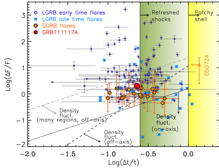
FIG. 8.— Relative variability flux ( \Delta F/F ) versus relative variability time scale ( \Delta t/t ) for a sample of short GRB X-ray flare candidates (orange filled circles; Margutti et al. 2011), as well as early (blue open diamonds; Chincarini et al. 2010) and late-time (light-blue stars; Bernardini et al. 2011) flares in long GRBs. A small black dot marks short GRBs with extended emission. The apparent flare detected in GRB 111117A is marked with a red filled circle. The late-time re-brightening detected in GRB 050724 is also shown for completeness with an orange open triangle. Solid, dashed and dot-dashed lines mark the kinematically allowed regions according to Ioka et al. (2005) (their equations (7) and (A2)).
