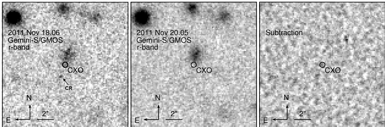
FIG. 2.— Gemini-South r -band observations of GRB 111117A at \delta t \approx 0.55 d (left) and \approx 2.54 d (middle). Digital image subtraction of the two observations (right) reveals no fading source coincident with the Chandra position (circle) or the host galaxy. We note that the apparent emission south-east of the Chandra position in the first epoch is a cosmic-ray (CR).
