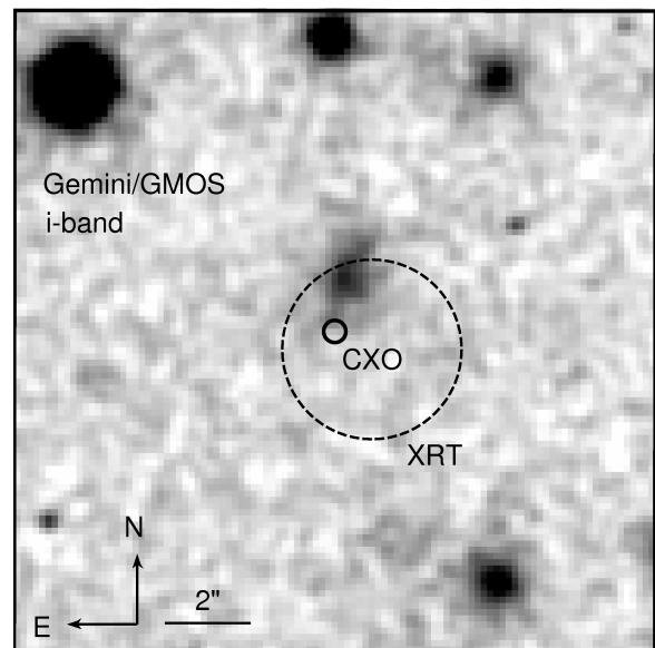
FIG. 3.— Gemini/GMOS i -band image of a 15'' \times 15'' field centered on the Chandra position of the X-ray afterglow of GRB 111117A (solid circle; 90% confidence region). Also shown is the Swift /XRT position (dashed circle; 90% confidence region). The host galaxy is clearly detected with an offset of about 1.25'' from the Chandra position.
