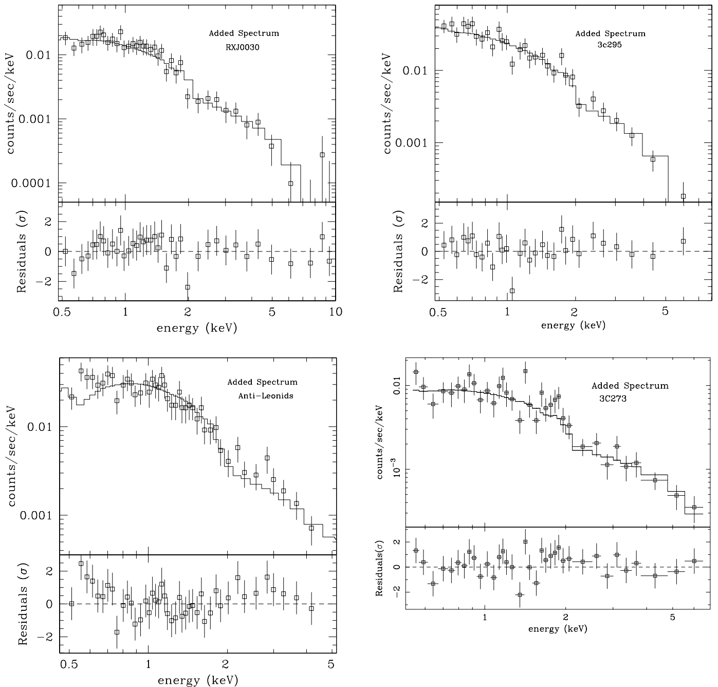
FIG. 5.—Added spectra of all the serendipitous sources (cluster and/or brightest sources excluded) in the RX J0030, 3C 295, anti-Leonid, and 3C 273 fields: best-fit spectra modeled with a single power law as given in Table 8. Data were binned in order to have an S/N > 3 in each energy bin.
