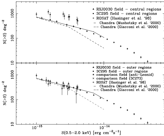
FIG. 2.— Upper panel: Chandra log N -log S between 0.5 and 2 keV measured in the RX J0030 and 3C 295 fields (only central chips, see text for details) compared with the 0.5–2 keV log N -log S measured by ROSAT (PSPC+HRI) from Hasinger et al. (1998) and Chandra “best-fit” results from Mushotzky et al. (2000) and Giacconi et al. (2000). In the Giacconi et al. log N -log S , the lack of sources for fluxes between 3 \times 10^{-15} and 10^{-14} ergs s^{-1} \text{ cm}^{-2} is attributed to cosmic variance (Giacconi et al. 2000). Reported fluxes for 3C 295 were increased by 1 \times 10^{-16} ergs \text{cm}^{-2} \text{ s}^{-1} for plotting clarity. Lower panel: Chandra log N -log S between 0.5 and 2 keV measured in the RX J0030 and 3C 295 fields (only outer chips) and log N -log S obtained in the two comparison fields (anti-Leonid: whole FOV; 3C 273: chip S3). ROSAT and Chandra deep-field data points are again plotted for comparison. Reported fluxes for 3C 273 were decreased by 10^{-16} ergs \text{cm}^{-2} \text{ s}^{-1} for plotting clarity.
