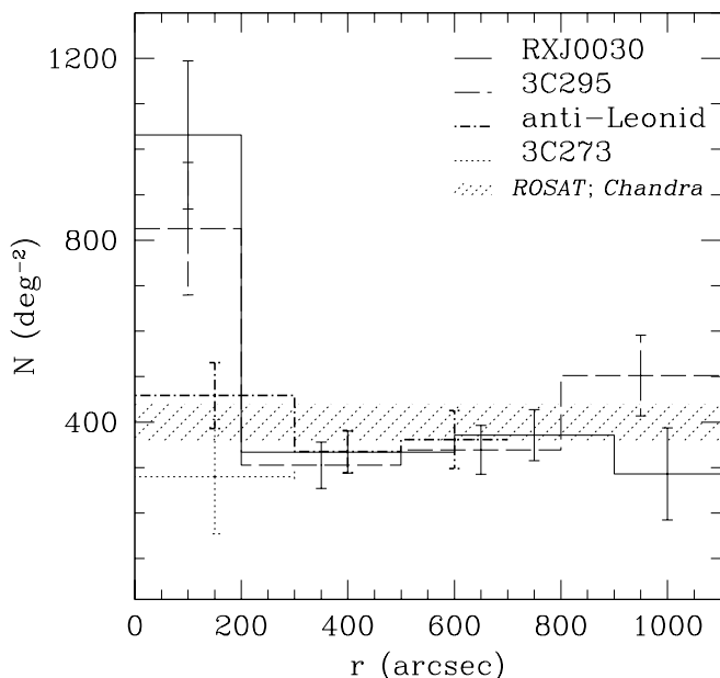
FIG. 4.—Radial distribution of the sources in RX J0030 (solid line), 3C 295 (dashed line), anti-Leonid (thick dash-dotted line), and 3C 273 (dotted line). At z = 0.5 , 200'' correspond to \sim 1.4 Mpc. The dashed area corresponds to the level of the ROSAT and Chandra log N -log S at a flux limit of 2.5 \times 10^{-15} ergs \text{cm}^{-2} \text{s}^{-1} .
