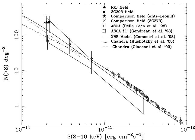
FIG. 3.— Chandra log N -log S between 2 and 10 keV measured for a flux limit of 2 \times 10^{-14} ergs \text{cm}^{-2} \text{ s}^{-1} in the RX J0030, 3C 295 (only central chips, see text for details), 3C 273 (S3 chip), and anti-Leonid fields (whole FOV, 4 chips). ASCA points (Cagnoni, Della Ceca, & Maccacaro 1998; Della Ceca et al. 2000), ASCA fluctuation limits (Gendreau, Barcons, & Fabian 1998), an AGN model for the XRB (Comastri et al. 1995), and Chandra deep-field “best-fit” results (calculated between 1 and 5 \times 10^{-14} ergs \text{cm}^{-2} \text{ s}^{-1} from Mushotzky et al. 2000; Giacconi et al. 2000) are plotted for comparison.
