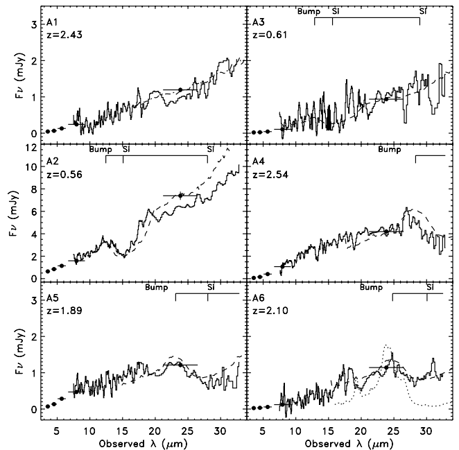
FIG. 1.— Observed spectra of sources A1–A6 in Table 1, smoothed to approximate resolution of individual IRS orders ( histograms ), with Mrk 231 AGN template showing silicate absorption at the listed redshift ( dashed curves ) or a QSO power law for source A1 without indication of silicate absorption ( dot-dashed curve ). Source A6 also shows the NGC 3079 starburst template ( dotted curve ) as an illustration that possible emission features in this spectrum are not fit by the PAH template. Filled circles : Fluxes and bandwidths of MIPS and IRAC measurements. The label “Si” shows the location of silicate absorption; the label “Bump” illustrates the location of the continuum peak at \sim 8 \mu\text{m} , which arises in a heavily absorbed source.
