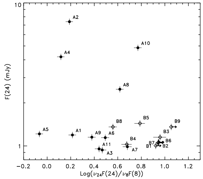
FIG. 11.—Comparison of f_\nu(24 \mu\text{m}) to infrared spectral slope as measured by \log [v f_\nu(24 \mu\text{m})/v f_\nu(8 \mu\text{m})] . Filled circles: AGNs in Table 1. Open circles: Starbursts in Table 2.
