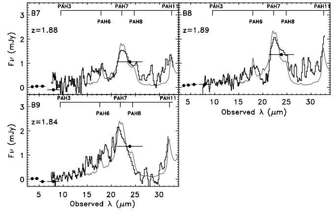
FIG. 4.—Observed spectra of sources B7–B9 in Table 2, smoothed to approximate resolution of individual IRS orders ( histograms ), with NGC 3079 starburst template at the redshift based on PAH emission features ( solid curves ). Filled circles same as in Fig. 1.
