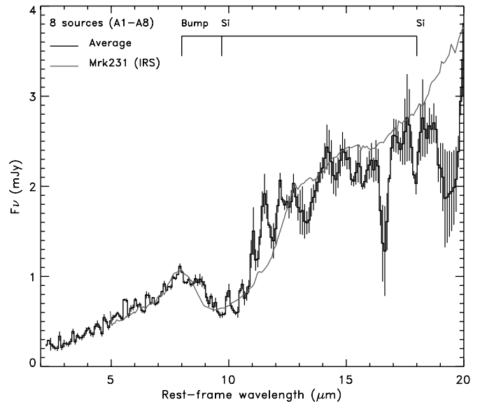
FIG. 9.—Histogram: Average rest-frame spectra of all AGN sources with redshifts in Table 1 normalized for flux density in interval 7.7\text{--}8.0 \mu\text{m} . Solid curve: Template of Mrk 231. Vertical bars: 1 \sigma uncertainties for the average spectrum.
