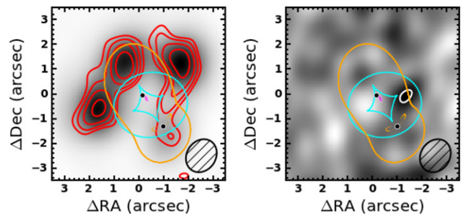
Figure 12. Left: SMA imaging (red contours, starting at 2\sigma and increasing by factors of 1.4) overlaid on the inverted, deconvolved map of the best-fit model visibilities (gray scale). The critical curve and caustics are represented by solid orange and cyan lines, respectively. The position of the lenses and the source are shown by plus signs and a magenta filled ellipse, respectively. The FWHM of the synthesized beam is shown in the lower right corner of each panel. Right: residual image (gray scale) obtained by inverting and deconvolving the residual visibilities (i.e., the difference between the model and data visibilities). Black and white contours indicate \pm 2\sigma level. A 2\sigma peak in the map of the residual visibilities may be an indication of additional minor structures in the lens plane or in the source plane.
