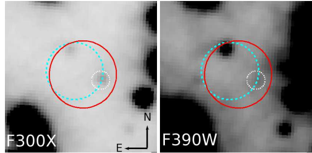
Figure 4. Finding chart of 47 Tuc I in the NUV. The solid red circles are the 3\sigma match circles for the radio position of the pulsar. They are centered on 47 Tuc I. The dashed cyan circles are the 3\sigma match circles of the Chandra source. The dashed white circles indicate the blue object that lies at 0''.12 from the pulsar. The images are 1''.0 \times 1''.0 in size.
