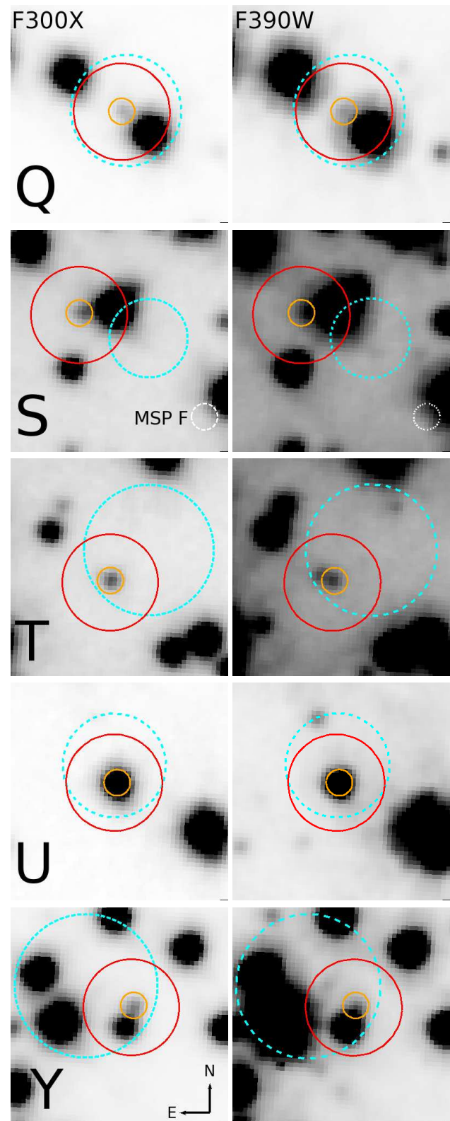
Figure 1. Finding charts of the companions to MSPs 47 Tuc Q, S, T, U and Y. Images in the filter F300X are shown on the left side while images in F390W are shown on the right. The solid red lines show the 3\sigma match circles centered on radio positions of the pulsars, which take into account the astrometric UVIS errors. The dashed cyan circles are the 3\sigma match circles of Chandra sources. The companion candidates are indicated by solid orange circles. Each image is 1''.0 \times 1''.0 in size.
