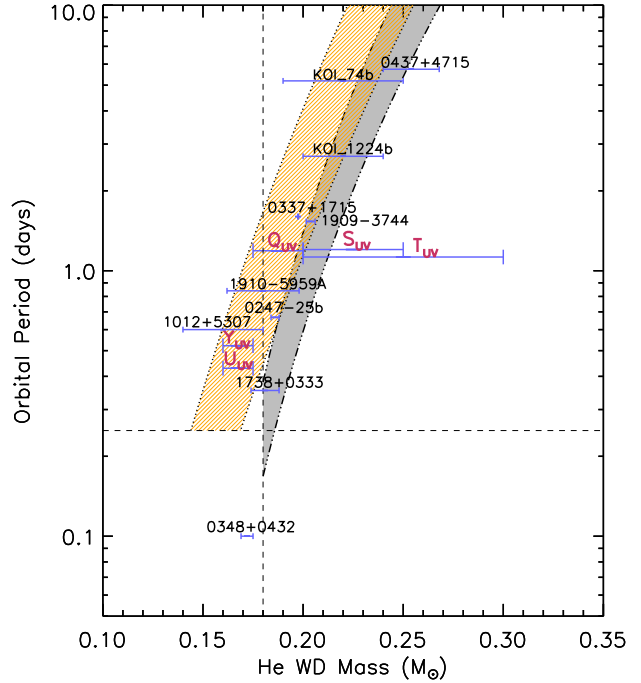
Figure 5. Mass-orbital period relations for He WDs. In gray is the relation as calculated by Tauris & Savonije (1999), with metallicities in the range Z = 0.001 - 0.02 (from right to left) and for WD masses in the range 0.18 - 0.45 M_{\odot} . In orange the relation by De Vito & Benvenuto (2010) for solar metallicity and for orbital periods > 0.25 d. The width of the relation corresponds to the uncertainties in its parameters. Overplotted are our results for the companions of 47 Tuc Q, S, T, U and Y. The error bars denote the possible masses for each object as determined from the WD cooling tracks by Serenelli et al. (2002). We also plot other pulsar companions for which 1\sigma uncertainties are less than 10% of the WD mass (see Tauris & van den Heuvel 2014 and references therein). The dashed vertical line denotes the lower mass limit ( 0.18 M_{\odot} ) for which the Tauris & Savonije (1999) relation is valid. The dashed horizontal line shows the minimum orbital period ( 0.25 d) for which the De Vito & Benvenuto (2010) relation is valid.
