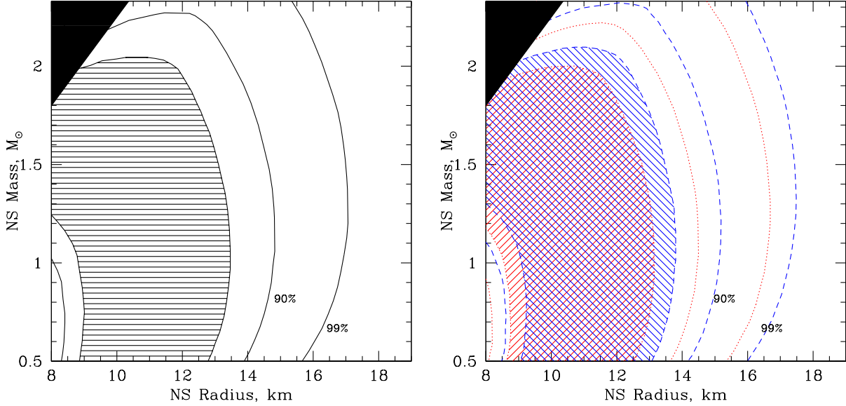
Figure 5. Left: Probability contours for the acceptable range of mass and radius for the \omega Cen qLMXB. This fit uses tbabs(nsatmos+pegpurlw) , with assumed distance of 5.3 kpc and a powerlaw photon index of 1.5. The solid black region at upper left identifies the excluded region (from causality constraints). The shaded region is the 1\sigma region, while the outer contours indicate the 90% and 99% confidence region. Right: Probability contours for the \omega Cen qLMXB, using the same assumptions as the left figure, except using assumed distances of 5.13 kpc (red, with / shading and dotted lines) or 5.47 kpc (blue, with \ shading and dashed lines).
