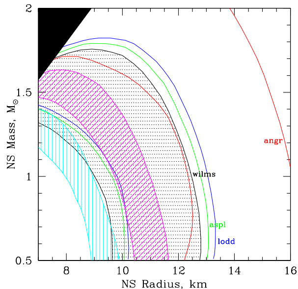
Figure 10. Six different 1\sigma probability contours for the acceptable range of mass and radius for the NGC 6397 qLMXB, depending on the abundance pattern chosen. This fit uses tbabs(spHe+pegwrlw) , with an assumed distance of 2.51 kpc and a powerlaw photon index of 1.5. The region shaded with black dots is the 1\sigma region for wilms abundances (Wilms, Allen & McCray 2000), as in Fig. 8. The blue and green contours enclose the (similar) 1\sigma regions for the aspl (Asplund et al. 2009) and lodd (Lodders 2003) abundance choices, and the red contours enclose this region for the angr (Anders & Grevesse 1989) abundances. The magenta contours (shaded at 45^\circ angle) are for a fixed column of 1.2 \times 10^{21} \text{ cm}^{-2} with wilms abundances, plus additional N_H at the cluster abundance; the cyan contours (shaded vertically) are the same, except the fixed column is at 1.0 \times 10^{21} \text{ cm}^{-2} .
