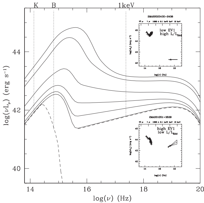
Figure 5. AGN spectral energy distribution predicted by the accretion disk and the corona model of Witt et al. (1997) for a black hole mass 10^8 M_{\odot} , viscosity parameter \alpha = 0.33 and from top to bottom L/L_{\text{Edd}} = 0.25, 0.1, 0.01, 0.003, 0.0017, 0.0013 respectively. Higher L/L_{\text{Edd}} give a more pronounced big blue bump relative to the X-rays and lower F(1 \text{ keV})/F_{B,R} ratios. Lower L/L_{\text{Edd}} produce a weaker big blue bump relative to the X-rays and higher F(1 \text{ keV})/F_{B,R} ratios. The dashed line shows the L/L_{\text{Edd}} = 0.0013 model reddened at optical/UV wavelengths by A_V = 3 (a reddening value obtained from IR/optical color modeling for 1051+3539, shown in lower insert; X-ray flux is left intrinsic since the Chandra X-ray flux was corrected for both Galactic and intrinsic absorption). Inserts show examples of red 2MASS AGN SEDs with high and low EV1 values.
