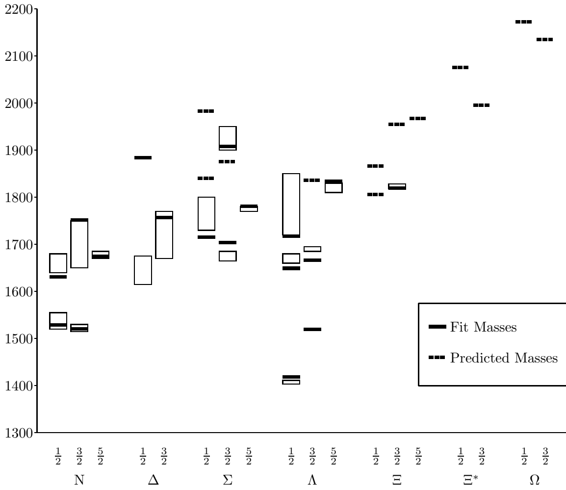
Figure 2. Masses of the L = 1 Baryons in the Quark Model; \chi^2 = 123.6432 , N_{fit} = 18
