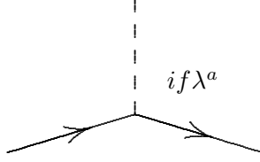
Figure 1. The constituent quark-Goldstone boson vertex of the chiral quark model. \lambda^a is a Gell-Mann flavor matrix.
