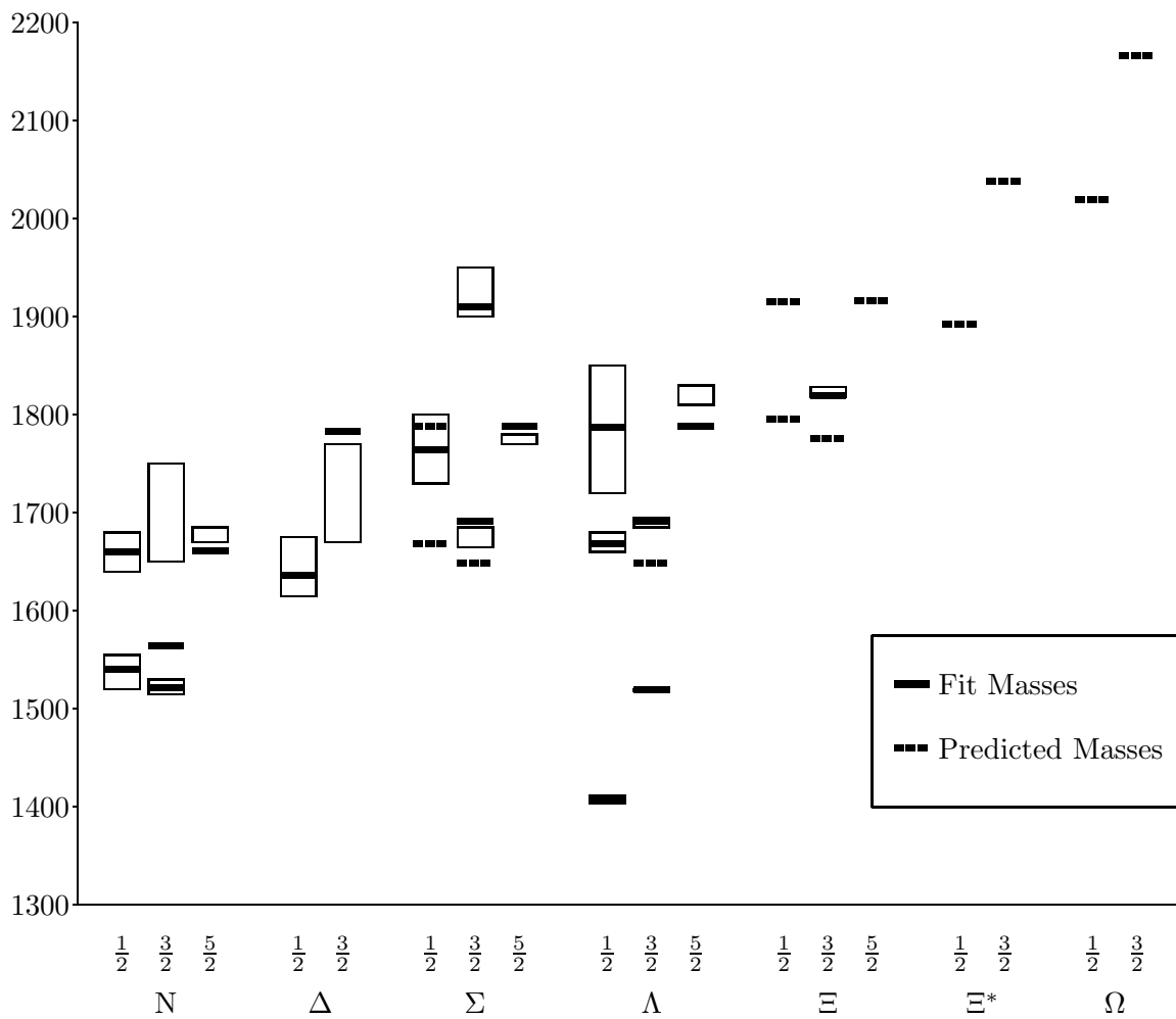
Figure 5. Masses of the L = 1 Baryons in the Chiral Quark Model with SU(3) Symmetric Interactions; \chi^2 = 33.2254 , N_{fit} = 18
