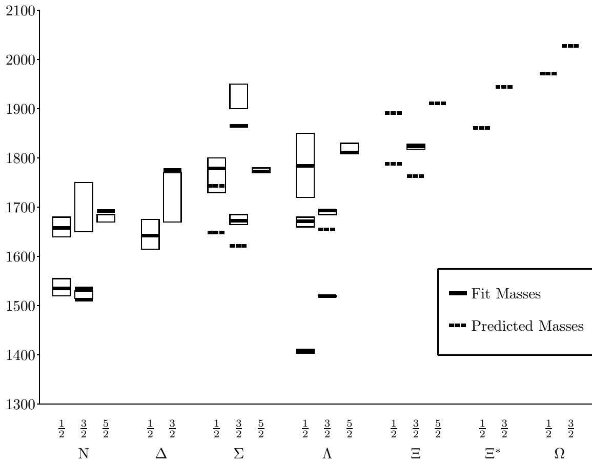
Figure 3. Masses of the L = 1 Baryons in the Chiral Quark Model; \chi^2 = 24.7568 , N_{fit} = 18
