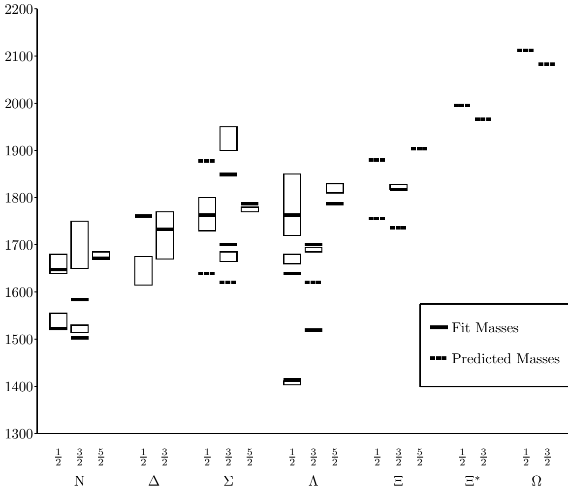
Figure 4. Masses of the L = 1 Baryons in the Quark Model with SU(3) Symmetric Interactions; \chi^2 = 79.2456 , N_{fit} = 18
