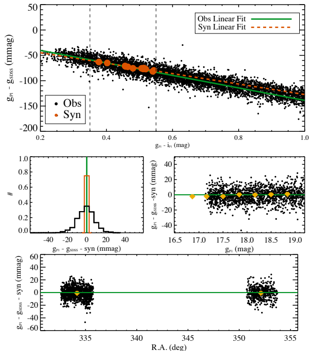
FIG. 2.— Visual representation of the steps of the Supercal method. The top panel shows the synthetic and observed differences in brightness of stars observed with the g_{SDSS} and g_{P1} band. Observed stars are shown in black and synthetic stars are shown in red. A linear transformation is fit to both the synthetic and observed trend. In the middle-left, a histogram is shown of the residuals from subtracting the synthetic trend from the observed stellar photometry. The histograms are normalized to unity. In the middle-right, the residuals as a function of magnitude are given. In the bottom panel, the dependency of the residuals on sky position is shown (bins given as yellow triangles).
