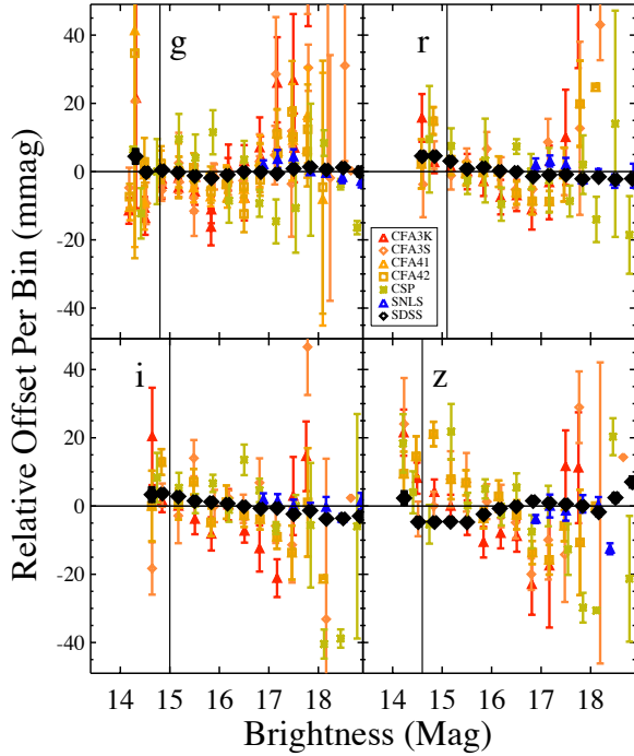
FIG. 5.— Relative offsets between stars in the PS1 sample and other samples as a function of apparent brightness in g_{P1}r_{P1}i_{P1}z_{P1} . The offsets shown are relative to the nominal Supercal correction given in Fig. 3. Comparisons for each survey are shown, and in black the offsets for SDSS are highlighted to quantify potential systematic uncertainties from the PS1 non-linearity. Vertical lines show where the PS1 sample is cut on the bright end.
