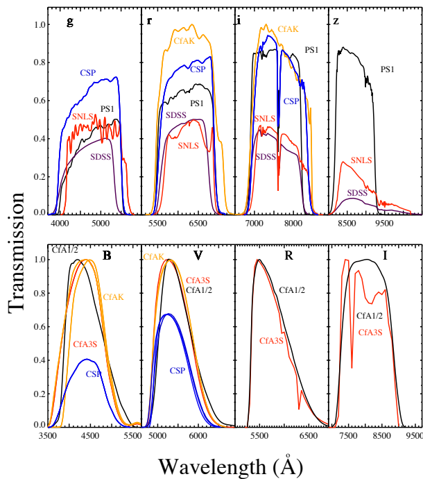
FIG. 1.— The filter transmission functions of all the systems in this analysis. Comparisons are broken into griz and BVRI . For both CSP and CfA-KeplerCam (CfAK), multiple filters are shown as in different periods of the survey, different filters were used.
