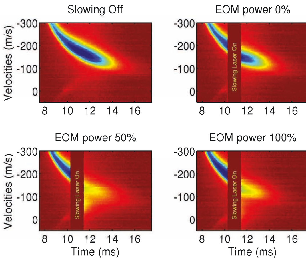
Figure 3.4.3: The velocity spectrum of the {}^6\text{Li} buffer-gas beam in the MOT center as a function of arrival time after YAG pulse. Blue corresponds to atomic signal. The dark red region labeled 'Slowing Laser On' represents the time window for the application of the slowing laser. Notice that very slow molecules are only seen immediately after the application of the slowing laser. This suggests that the slowing only occurs in the longitudinal distance immediately before the MOT center.
