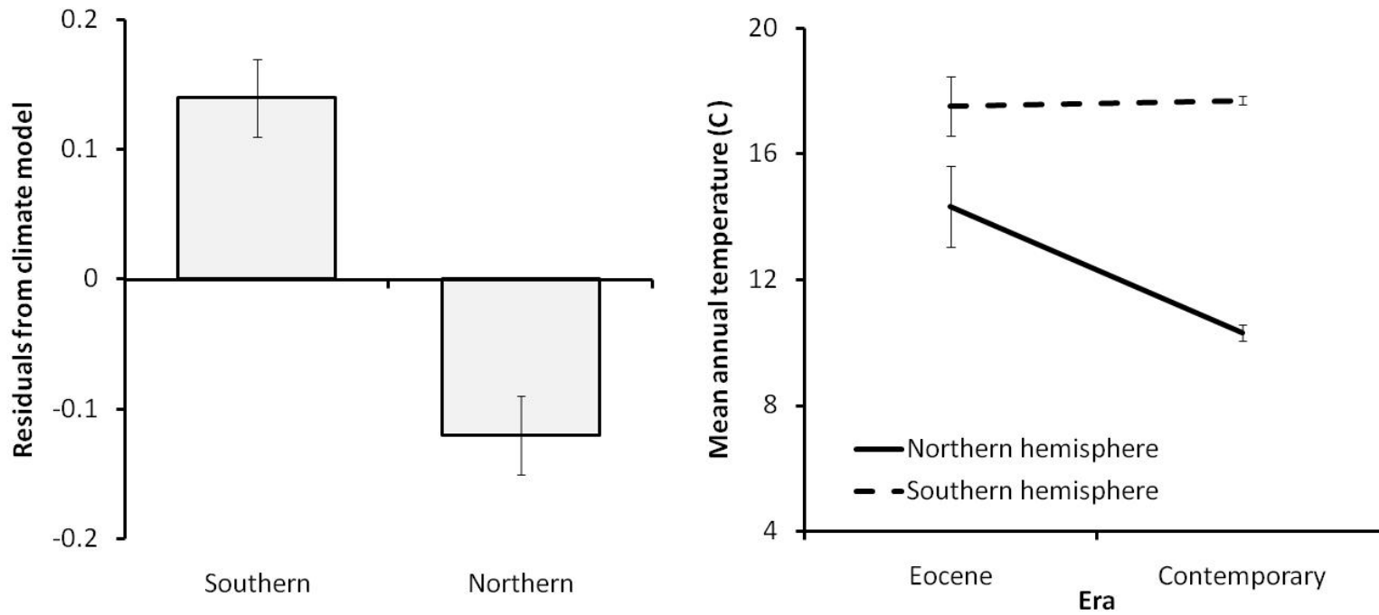
6 Figure 3. Residuals of model 1 (climate variables only) plotted by hemisphere for all data (a) and average mean annual temperature 7 fore the southern and northern hemispheres on the basis of the contemporary and Eocene data. Bars = standard error of the mean.
