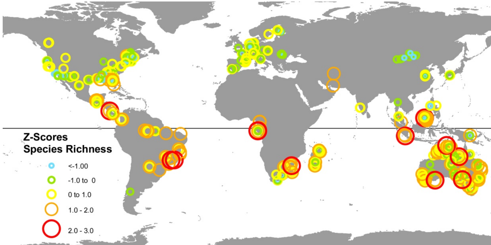
Figure 1. Species richness of sites considered in this study. Warmer colors and larger circles are more diverse. Each point indicates one site. Sites are divided into richness quintiles. Black line indicates the equator and hence divides the northern and southern hemispheres.
