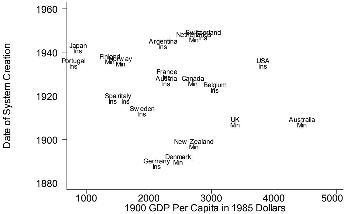
Figure 4 (a): Date and Type of OAI System Adopted, and GDP Per Capita in 1900 'Ins' denotes an Insurance System, 'Min' a Minimum system.
