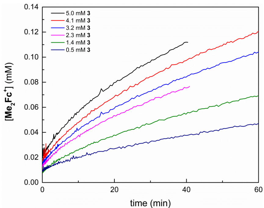
Figure 2.81. [\text{Me}_2\text{Fc}^+] vs. time for reaction of \text{Me}_2\text{Fc} (0.5 mM) with o -chloranil (0.5 mM) with increasing [\mathbf{3}] .
