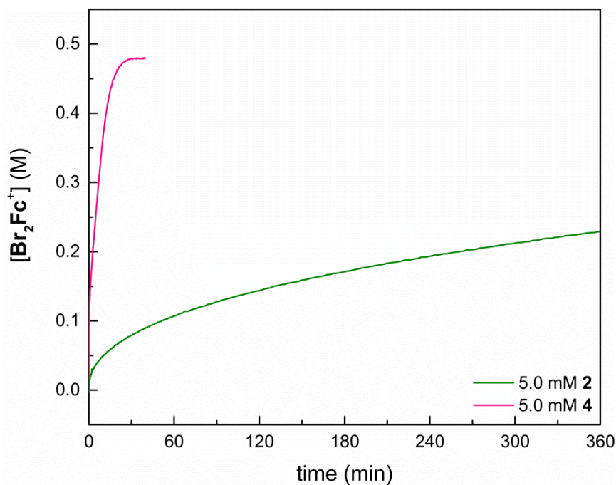
Figure 2.86. [\text{Br}_2\text{Fc}^+] vs. time for reaction of \text{Br}_2\text{Fc} (0.5 mM) with o -chloranil (2.5 mM), mediated by 2 (5.0 mM) and 4 (5.0 mM), in \text{CH}_2\text{Cl}_2 at 25 °C, under an atmosphere of nitrogen.
