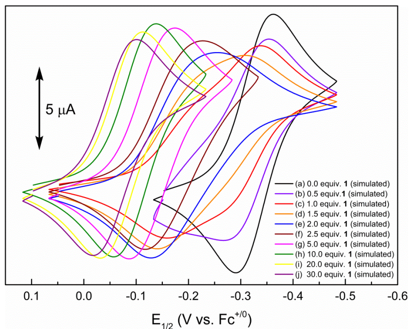
Figure 2.33. Full set of CEC simulations of CV data for o -chloranil (initial concentration = 0.5 mM) recorded in 0.1 M n\text{Bu}_4\text{NBArF}_{24}/\text{CH}_2\text{Cl}_2 (glovebox) in the presence of increasing [1].
