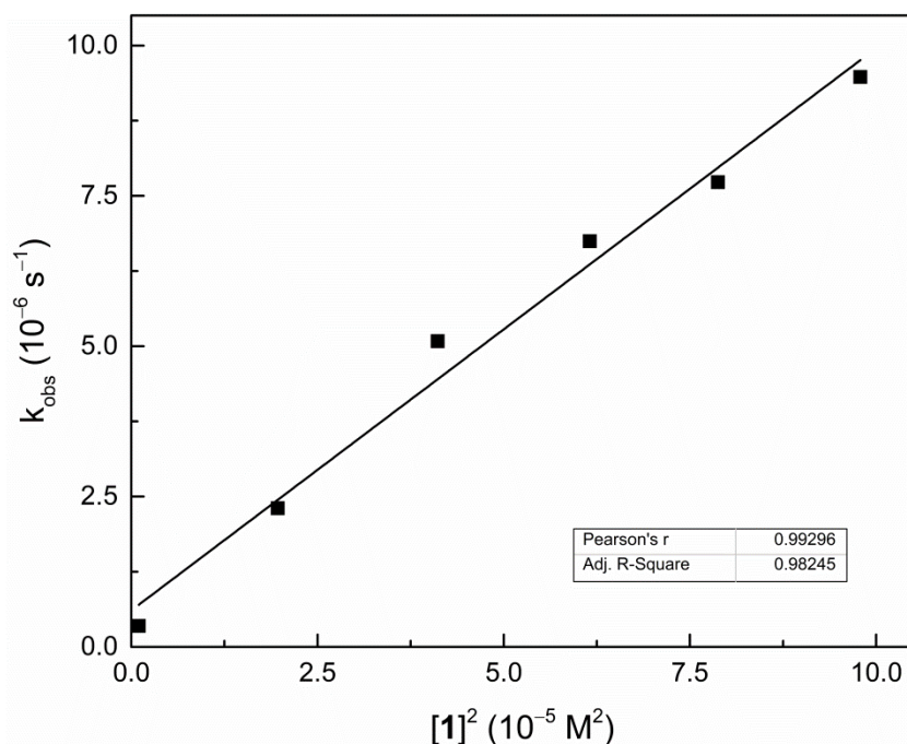
Figure 2.64. Second order plot of initial rate constants ( k_{\text{obs}} ) vs. [1]^2 for electron transfer from BrFc (1.0 mM) to Q (1.0 mM), promoted by 1 (1.0–10.0 mM) in \text{CH}_2\text{Cl}_2 at 25 °C under \text{N}_2 ( R^2 = 0.98245 ).
