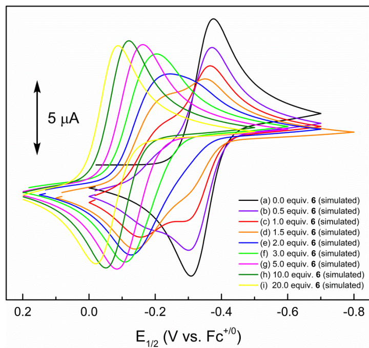
Figure 2.47. Full set of simulations of CV data for o -chloranil (initial concentration = 0.5 mM) recorded in 0.1 M n\text{Bu}_4\text{NBArF}_{24}/\text{CH}_2\text{Cl}_2 (glovebox) in the presence of increasing [6]
