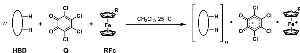
Figure 2.62. Homogeneous electron transfer between \text{Q} and ferrocene derivatives (RfC) promoted by HBDs.
