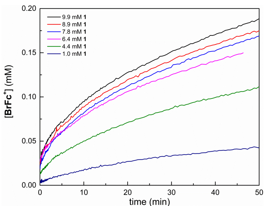
Figure 2.77. [BrFc + ] vs. time for reaction of BrFc (1.0 mM) with o -chloranil (1.0 mM), with increasing [1], for two runs.
