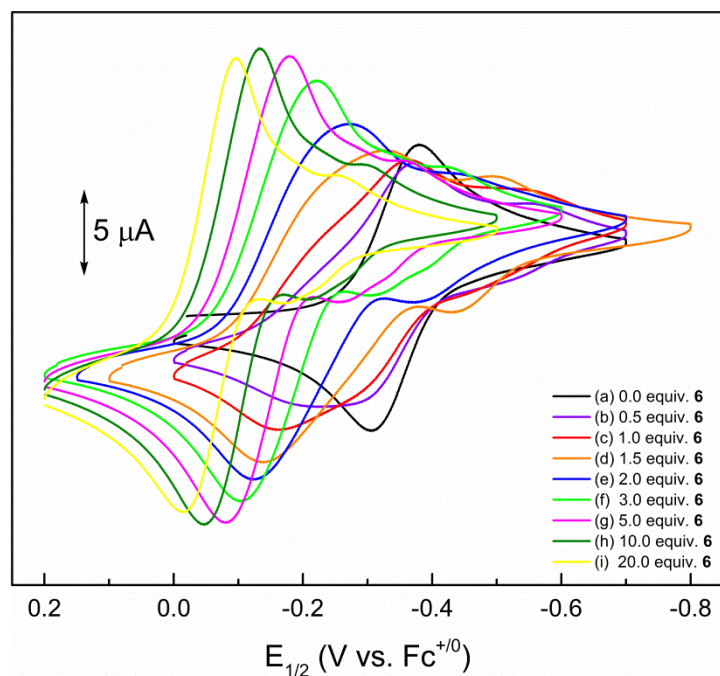
Figure 2.46. Full set of experimental CVs of o -chloranil (initial concentration = 0.5 mM) recorded in 0.1 M n\text{Bu}_4\text{NBArF}_{24}/\text{CH}_2\text{Cl}_2 (glovebox) in the presence of increasing [6]. In scans (b)–(i), the additional current peaks at lower potentials are attributed to the 2e^- reduction.
