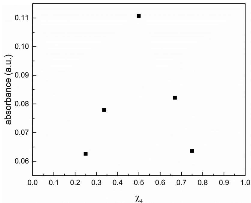
Figure 2.68. Job plot using absorbance of MePTZ + obtained after reaction between MePTZ (0.4 mM) and Q in the presence of 4 in CH 2 Cl 2 at 25 °C under N 2 . The total concentration of [ Q ] + [ 4 ] was held at 0.2 mM. [Note: the y-axis is scaled and does not start at 0].
