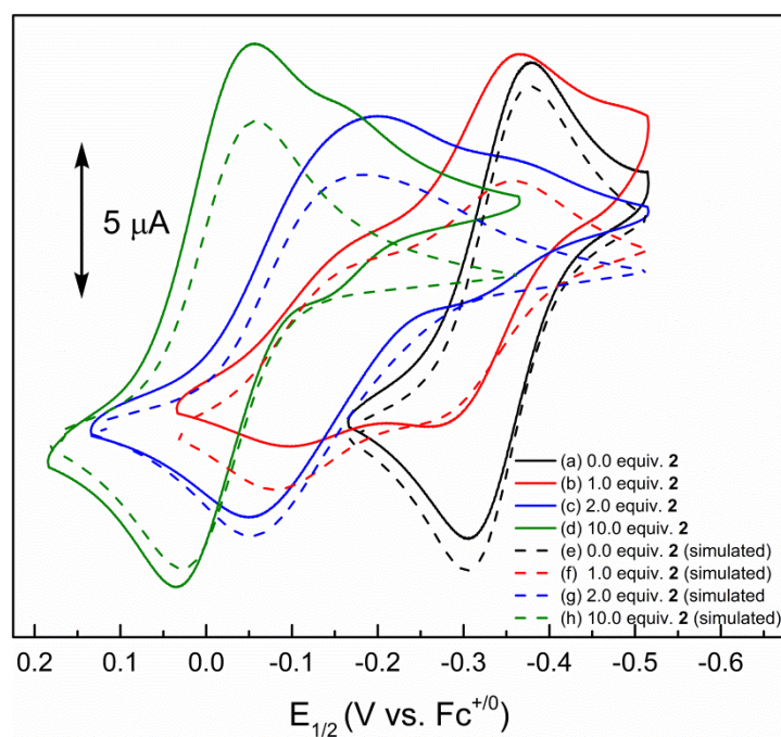
Figure 2.13. Experimental CVs of o -chloranil (initial concentration = 0.5 mM) recorded in 0.1 M n\text{Bu}_4\text{NBARF}_{24}/\text{CH}_2\text{Cl}_2 (glovebox) in the presence of increasing [2] and comparison with simulation of a CEC mechanism. In scans (c) and (d), the additional current peaks at lower potential are attributed to the 2e^- reduction.
