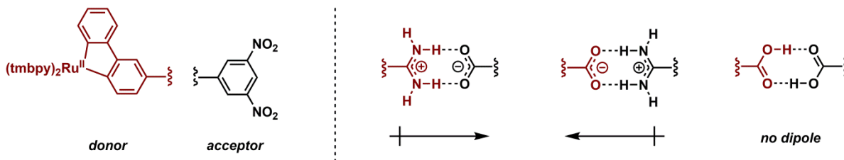
Figure 1.7. Photoinduced electron transfer across salt bridges. 17a
