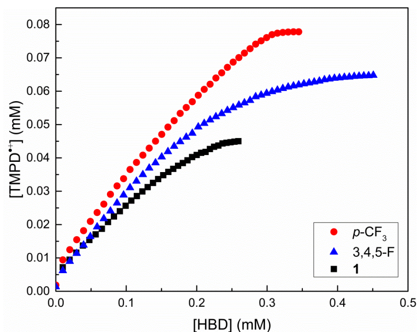
Figure 2.92. Titration of TMPD (0.1 mM) and p -fluoranil (0.1 mM) using 1 and two benzamide-substituted guanidinium salts. Formation of \text{TMPD}^{\bullet+} (at 567 nm) was monitored by UV-vis spectrophotometry.
