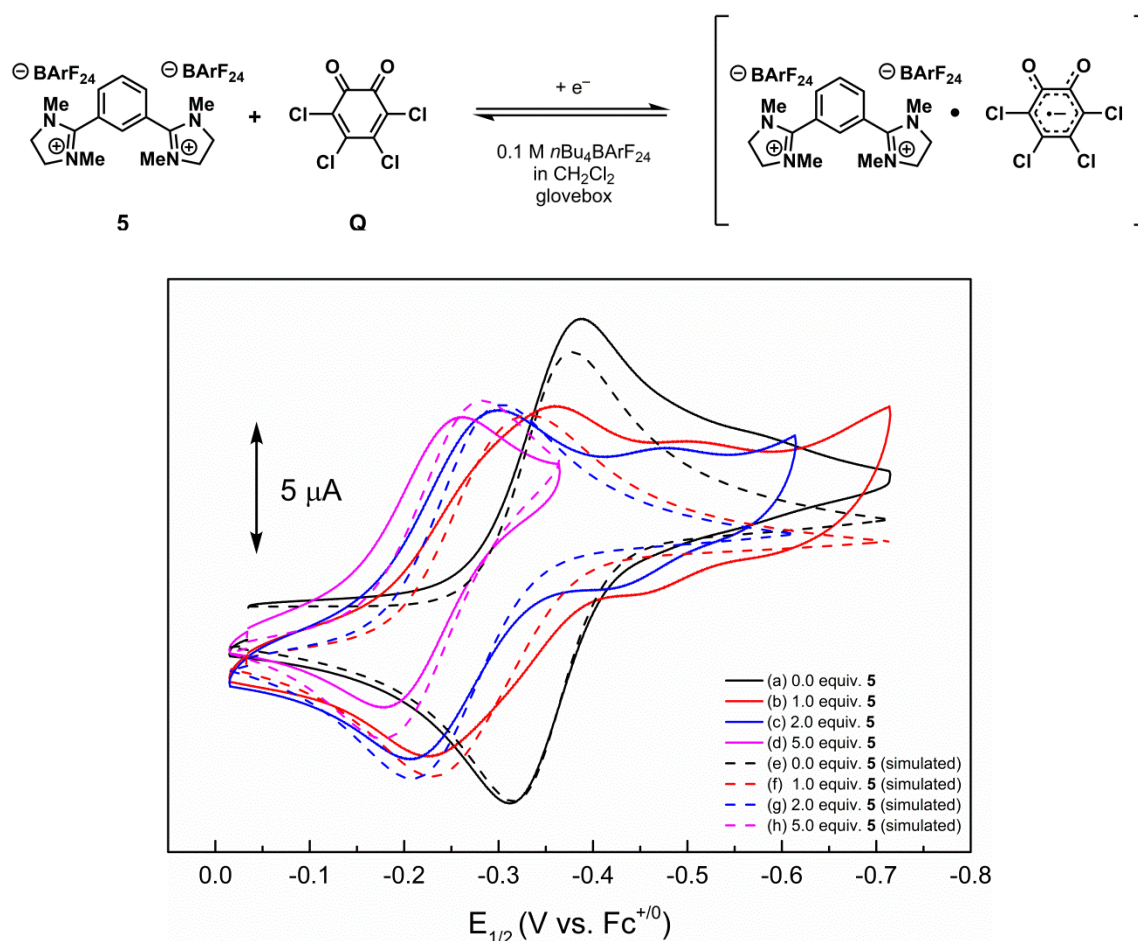
Figure 2.21. Experimental CVs of o -chloranil (initial concentration = 0.5 mM) recorded in 0.1 M n Bu 4 NBARF 24 /CH 2 Cl 2 (glovebox) in the presence of increasing [ 5 ] and comparison with simulation of an EC mechanism. In scans (b) and (c), the additional current peaks at lower potential are attributed to the 2e - reduction.
