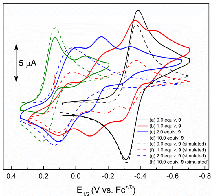
Figure 2.29. Experimental CVs of o -chloranil (initial concentration = 0.5 mM) recorded in 0.1 M n\text{Bu}_4\text{NBARF}_2 / \text{CH}_2\text{Cl}_2 (glovebox) in the presence of increasing [9] and comparison with simulation of a CEC mechanism. In scans (b)–(d), the additional current peaks at lower potential are attributed to the 2e^- reduction.
