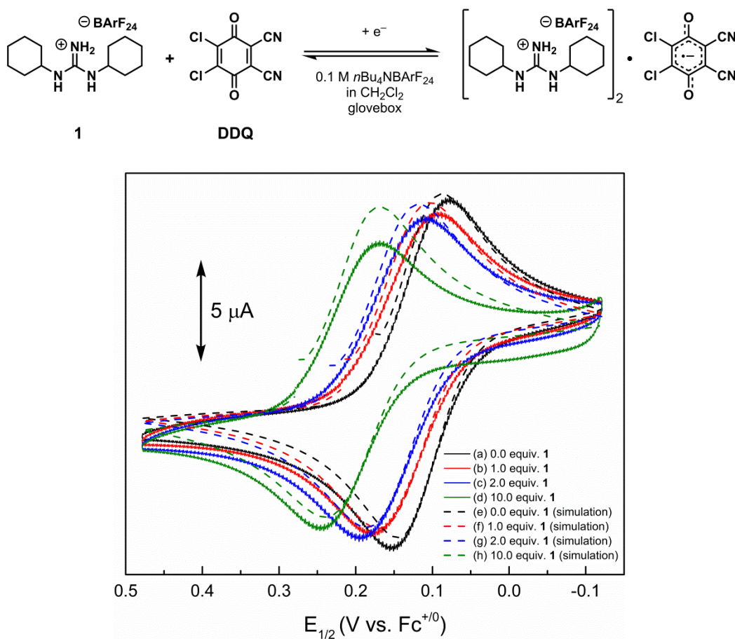
Figure 2.95. Experimental CVs of DDQ (initial concentration = 0.5 mM) recorded in 0.1 M n\text{Bu}_4\text{NBARF}_{24}/\text{CH}_2\text{Cl}_2 (glovebox) in the presence of increasing [ 1 ] and comparison with simulation of an ECC mechanism.
