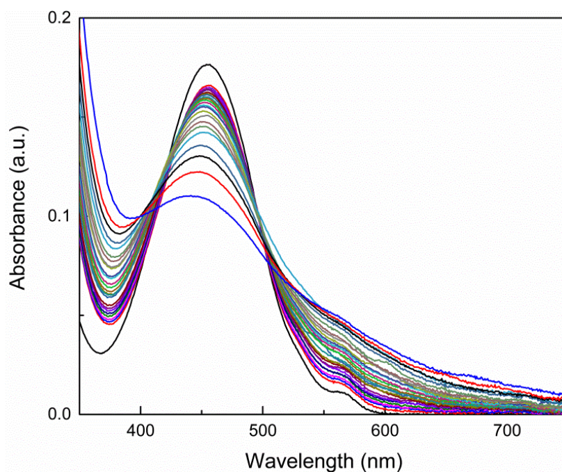
Figure 2.60. Absorbance vs. wavelength data for titration of o -chloranil with increments of 4 .
