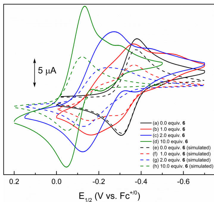
Figure 2.23. Experimental CVs of o -chloranil (initial concentration = 0.5 mM) recorded in 0.1 M n\text{Bu}_4\text{NBARF}_{24}/\text{CH}_2\text{Cl}_2 (glovebox) in the presence of increasing [ 6 ] and comparison with simulation of a CEC mechanism. In scans (b)–(d), the additional current peaks at lower potential are attributed to the 2e^- reduction.
