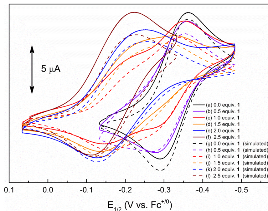
Figure 2.11. Experimental CVs of o -chloranil (initial concentration = 0.5 mM) recorded in 0.1 M n\text{Bu}_4\text{NBArF}_{24}/\text{CH}_2\text{Cl}_2 (glovebox) in the presence of increasing [1] and comparison with simulation of a CEC mechanism. Only data collected at low [1] are shown.
