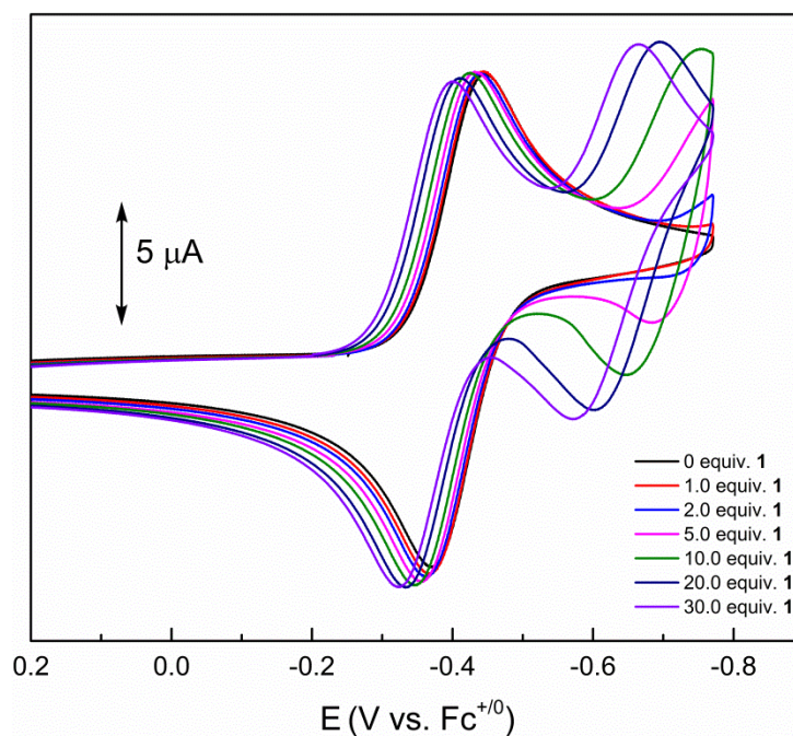
Figure 2.5. Experimental CVs of p -chloranil (initial concentration = 0.5 mM) recorded in 0.1 M n Bu 4 PF 6 /CH 2 Cl 2 (glovebox) in the presence of increasing [1].
