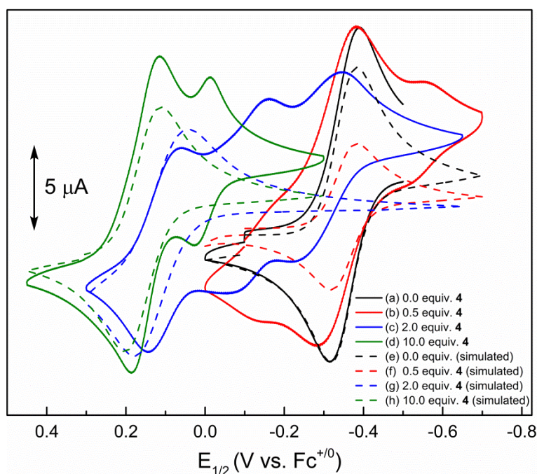
Figure 2.20. Experimental CVs of o -chloranil (initial concentration = 0.5 mM) recorded in 0.1 M n Bu 4 NBArF 24 /CH 2 Cl 2 (glovebox) in the presence of increasing [4] and comparison with simulation of a CE mechanism. In scans (b)–(d), the additional current peaks at lower potential are attributed to the 2e − reduction.
