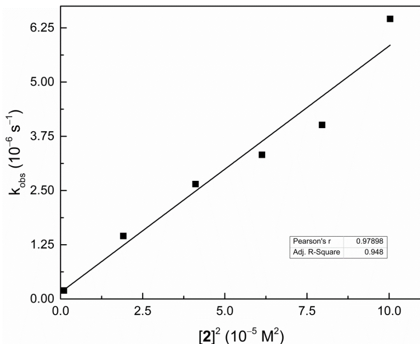
Figure 2.65. Second-order plot of initial rate constants ( k_{\text{obs}} ) vs. [\mathbf{2}]^2 for electron transfer from Br 2 Fc (1.0 mM) to Q (1.0 mM), promoted by 2 (1.0–10 mM) in \text{CH}_2\text{Cl}_2 at 25 °C under \text{N}_2 ( R^2 = 0.948 )
