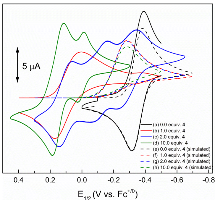
Figure 2.43. Experimental CVs of o -chloranil (initial concentration = 0.5 mM) recorded in 0.1 M n\text{Bu}_4\text{NBArF}_{24}/\text{CH}_2\text{Cl}_2 (glovebox) in the presence of increasing [4] and comparison with simulation of an EC mechanism representing a poor fit.
