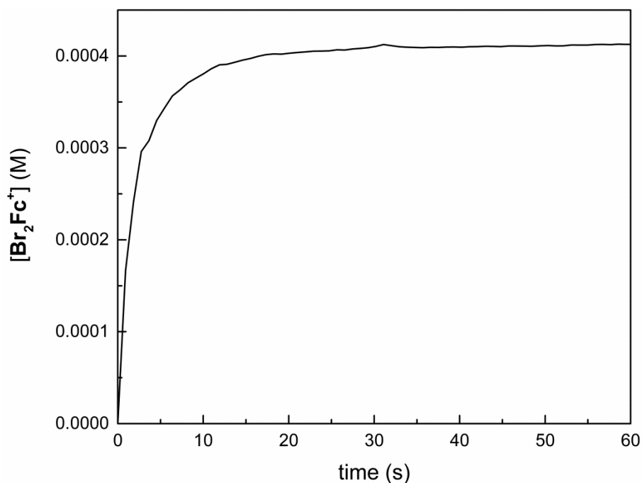
Figure 2.69. Raw data for electron transfer from Br 2 Fc (0.5 mM) to o -chloranil (2.5 mM) promoted by 9 (5.0 mM), in CH 2 Cl 2 at 25 °C.
