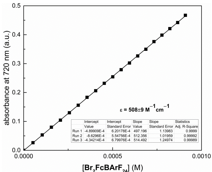
Figure 2.73. Beer's Law Plot for \text{Br}_2\text{FcBARF}_{24} at 720 nm. The average of three runs is shown.
