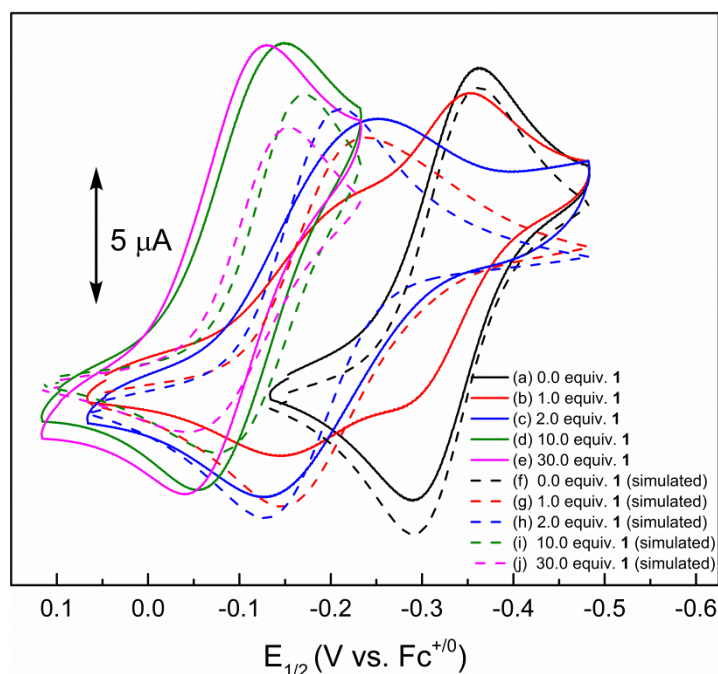
Figure 2.35. Experimental CVs of o -chloranil (initial concentration = 0.5 mM) recorded in 0.1 M n\text{Bu}_4\text{NBArF}_{24}/\text{CH}_2\text{Cl}_2 (glovebox) in the presence of increasing [1] and comparison with simulation of an ECC mechanism representing a poor fit.
