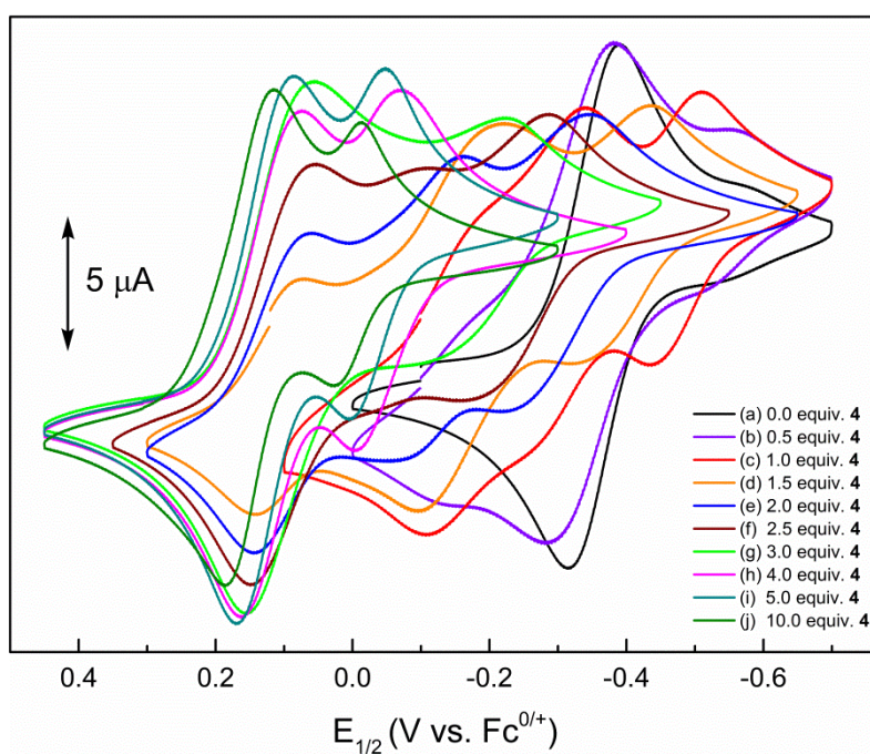
Figure 2.41. Full set of experimental CVs of 0.5 mM o -chloranil recorded in 0.1 M n Bu 4 NBArF 24 /CH 2 Cl 2 (glovebox) in the presence of increasing [ 4 ]. In scans (b)–(j), the additional current peaks at lower potential are attributed to the 2e − reduction.
