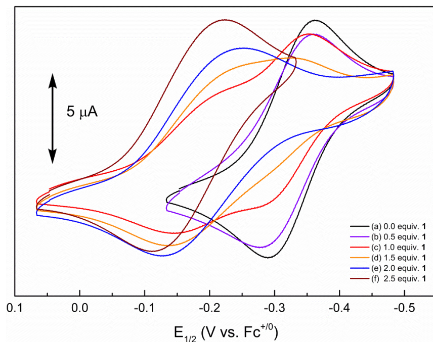
Figure 2.8. Experimental CVs of o -chloranil (initial concentration = 0.5 mM) recorded in 0.1 M n Bu 4 NBArF 24 /CH 2 Cl 2 (glovebox) in the presence of increasing [ 1 ]. Only data collected at low [ 1 ] are shown.
