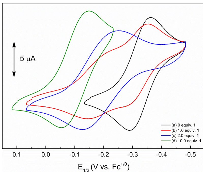
Figure 2.7. Experimental CVs of o -chloranil (initial concentration = 0.5 mM) recorded in 0.1 M n\text{Bu}_4\text{NBARF}_{24}/\text{CH}_2\text{Cl}_2 (glovebox) in the presence of increasing [1].
