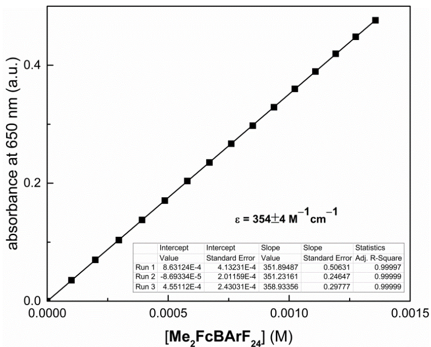
Figure 2.74. Beer's Law Plot for \text{Me}_2\text{FcBARF}_{24} at 650 nm. The average of three runs is shown.
