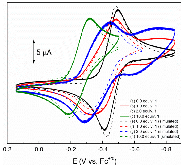
Figure 2.93. Experimental CVs of p -chloranil (initial concentration = 0.5 mM) recorded in 0.1 M n Bu 4 NBArF 24 /CH 2 Cl 2 (glovebox) in the presence of increasing [1] and comparison with simulation of an ECC mechanism.
