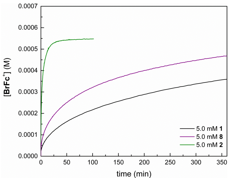
Figure 2.85. [\text{BrFc}^+] vs. time for reaction of \text{BrFc} (0.5 mM) with o -chloranil (2.5 mM), mediated by 1 (5.0 mM), 2 (5.0 mM), and 8 (5.0 mM), in \text{CH}_2\text{Cl}_2 at 25 °C, under an atmosphere of nitrogen.
