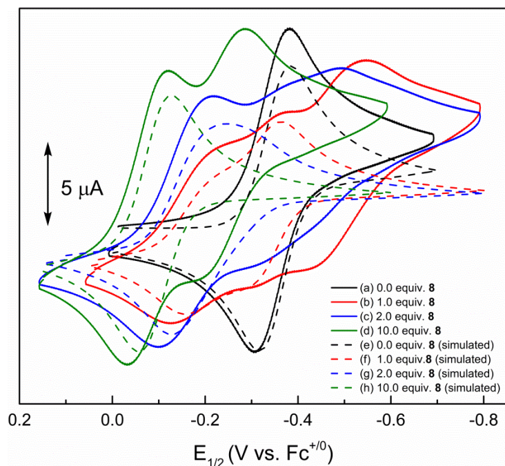
Figure 2.27. Experimental CVs of o -chloranil (initial concentration = 0.5 mM) recorded in 0.1 M n\text{Bu}_4\text{NBARF}_{24}/\text{CH}_2\text{Cl}_2 (glovebox) in the presence of increasing [8] and comparison with simulation of a CEC mechanism. In scans (b)–(d), the additional current peaks at lower potential are attributed to the 2e^- reduction.
