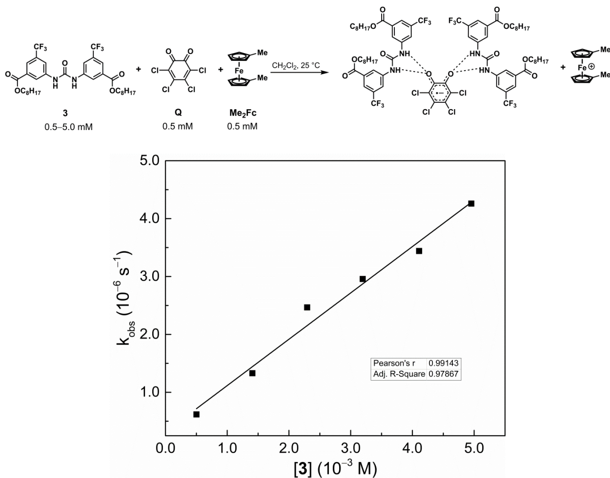
Figure 2.66. First-order plot of initial rate constants ( k_{\text{obs}} ) vs. [ 3 ] for electron transfer from \text{Me}_2\text{Fc} (0.5 mM) to Q (0.5 mM), promoted by 3 (0.5–5.0 mM) in \text{CH}_2\text{Cl}_2 at 25 °C under \text{N}_2 ( R^2 = 0.97867 )
