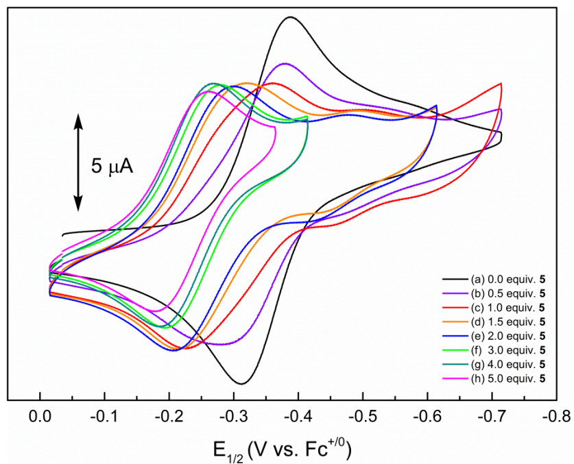
Figure 2.44. Full set of experimental CVs of o -chloranil (initial concentration = 0.5 mM) recorded in 0.1 M nBu_4NBArF_{24}/CH_2Cl_2 (glovebox) in the presence of increasing [5]. In scans (b)–(d), the additional current peaks at lower potential are attributed to the 2e^- reduction.
