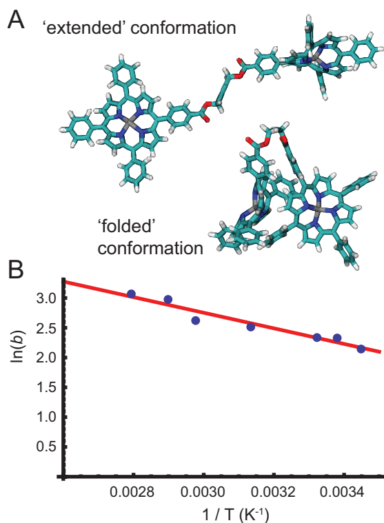
Figure 6. (A) Models of ‘extended’ and ‘folded’ conformations of the zinc porphyrin tweezer from the UFF structure optimizations. (B) Van’t Hoff Plot of the parameter \ln(b) versus inverse temperature, where b is the ratio of H- to J-dimer population. Blue dots are the values of b obtained from the optimizations to the linear absorption and 2D FS spectra over the full range of temperatures shown in Fig. 5. The linear fit to these points (red line) yields the standard state change in entropy and enthalpy associated with the ‘extended’-to-‘folded’ conformational transition, \Delta S_a^\circ = 55.5 \text{ J mol}^{-1} \text{ K}^{-1} and \Delta H_a^\circ = 10.9 \text{ kJ mol}^{-1} , respectively.
