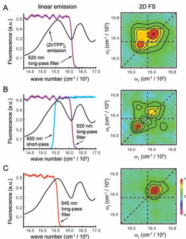
Figure 3. (A) Left panel: The transmission spectrum of a 620 nm long-pass filter (purple) is shown superimposed with the emission spectrum (black) of (ZnTPP) 2 at 23 °C while exciting at 570 nm near the red edge of the Q(0,1) band. This filter passes the majority of the lowest-energy
