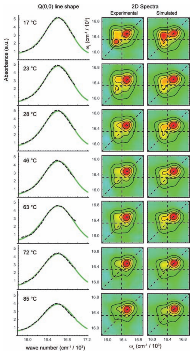
Figure 5. Left column: The linear absorption spectrum of the Q(0,0) band of (\text{ZnTPP})_2 dimers in DSPC liposomes (dashed black) is overlaid with its optimized fit (green) for each of the seven temperatures investigated. Right column: The real part of the 2D FS total correlation spectra is compared to its optimized fit for each temperature. As the temperature is increased, the red-shifted diagonal peak and the above diagonal cross peak decrease in intensity, corresponding to a loss in the relative population of J-dimer conformation. These temperature-dependent changes in
