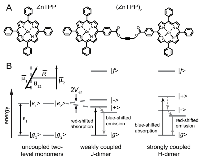
Figure 1. (A) Structures of the chromophores used in this study, zinc tetraphenylporphyrin (ZnTPP) and a covalently linked dimer of ZnTPP (ZnTPP) 2 . (B) Energy level diagrams of two degenerate two-level molecules. Electronic coupling results in a four-level dimer with a single ground state |g\rangle , two non-degenerate singly-excited states |\pm\rangle , and a doubly-excited state |f\rangle . For a ‘weakly coupled J-dimer’ (i.e., with a head-to-tail dipole arrangement), the |+\rangle state is shifted to lower energy. The situation is juxtaposed for a ‘strongly coupled H-dimer’ (i.e., a side-by-side dipole arrangement). Because transitions involving the |+\rangle state are favored, absorption is red-shifted for a J-dimer, while it is blue-shifted for an H-dimer. After excited state relaxation, emission occurs from the lowest-energy singly-excited state, which is lower in energy for the H-dimer than the J-dimer due to the H-dimer’s stronger coupling. Therefore, fluorescence from the H-dimer occurs on the red edge of the emission line shape while emission from the J-dimer occurs on the blue edge of the emission line shape.
