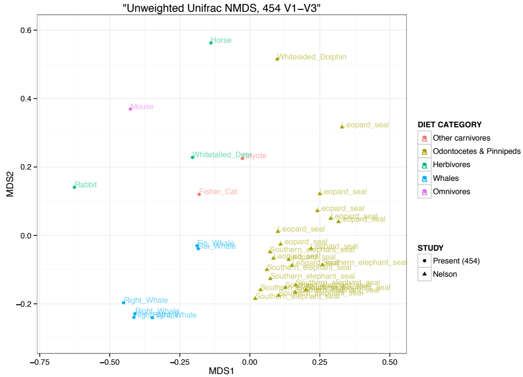
Fig. A2.10: NMDS ordination of unweighted UniFrac distances for pinniped samples from Ref. 38 and the present study. Distances based on 97% OTUs clustered from 454 sequencing of the V1-V3 region of the bacterial 16S rRNA gene.
