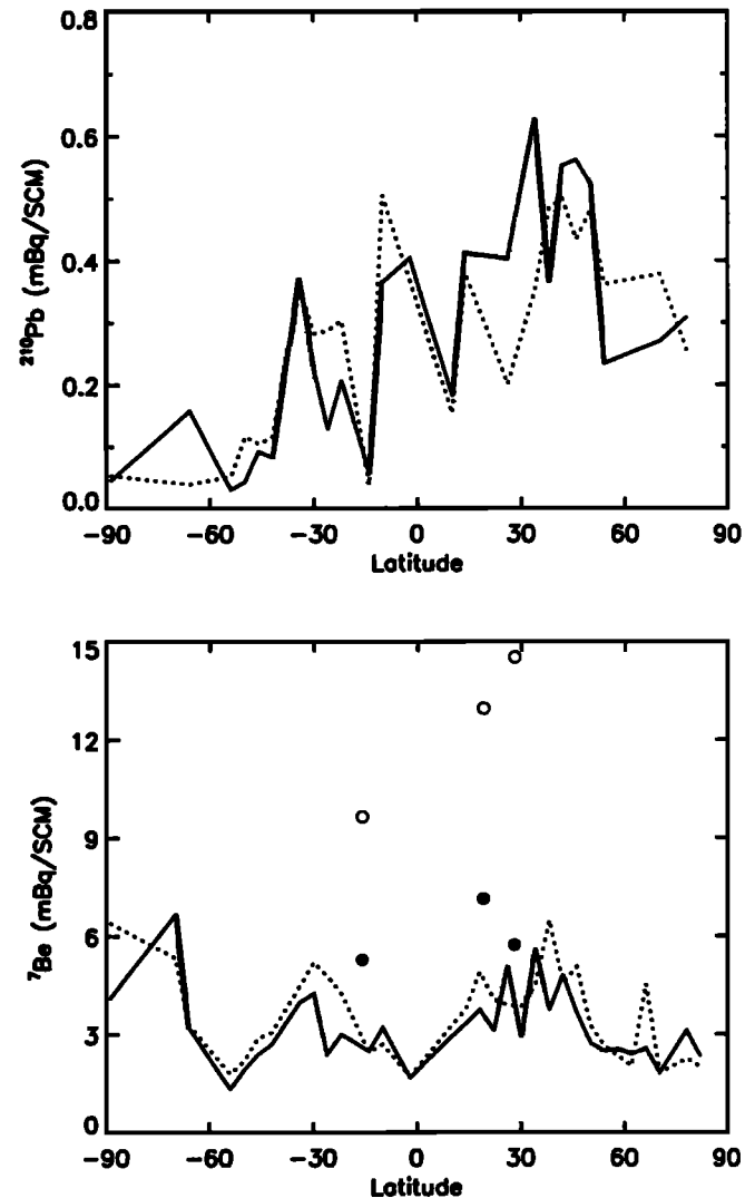
Figure 7. Observed (solid line) and simulated (dotted line) annual average surface concentrations of ^{210}\text{Pb} (47 sites) and ^7\text{Be} (91 sites) as a function of latitude. The data from individual sites are averaged over 4^\circ latitudinal bins. The observations are for the ensemble of years available (K96). Model results are for 1994. Symbols show the observed (dots) and model (circles) annual average ^7\text{Be} surface concentrations at three mountain sites (Tenerife, Mauna Loa, and Chacaltaya).
