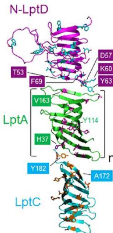
Figure 9. Proposed structure of the Lpt trans-envelope bridge. When pBPA is placed at the indicated positions in N-LptD, LptA, or LptC, UV-induced crosslinking can be observed between the mutagenized protein and its contact partner. The N-LptD structure is a predicted structure. Figure taken directly from Freinkman et al 103 . Copyright 2012, American Chemical Society.
