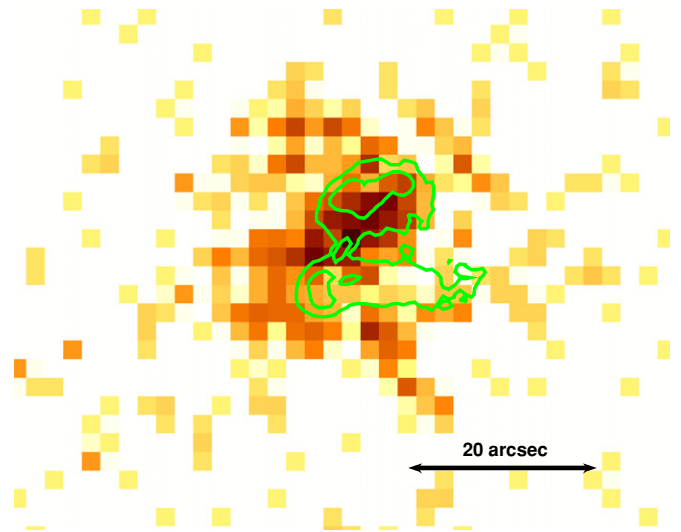
Figure 2. Chandra /ACIS-S image of 3C 288 in the 0.23–0.50 keV soft X-ray band with 5 GHz radio contours (0.6 resolution) overlaid. This image shows the soft X-ray excess, which is not commonly observed in clusters of galaxies and is uniformly detected across the whole 42 ks observation.
