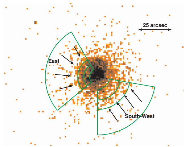
Figure 4. Gaussian-smoothed ( \text{radius}_{\text{FWHM}} = 2'' ) Chandra /ACIS-S image in the 0.23–2.50 keV band. The image has 2'' bins. The black sets of arrows denote the positions of two surface brightness discontinuities. The image also shows regions where surface brightness profiles were fitted and where spectra were extracted for temperature measurements. A large 1' region centered on the radio galaxy was used for global temperature and abundance measurements. The surface brightness profiles shown in Figures 5 and 6 are taken from the two sectors.
