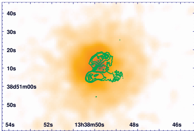
Figure 1. Gaussian-smoothed (radius FWHM = 2''), exposure-corrected, background-subtracted Chandra /ACIS-S image of 3C 288 in the 0.5–2.5 keV band. All point sources, other than the active nucleus of 3C 288, have been removed. We see diffuse thermal emission with a temperature of \sim 3 keV extending to \sim 510 kpc ( \sim 1.73 ). Contours from the 4.9 GHz radio map of 3C 288 are overlaid and 10 contour levels are placed linearly between 0.4 and 12.0 mJy beam -1 . The radio source is small, 294 kpc (1.3 across), and the radio core is coincident with the optical host galaxy. A peak of X-ray emission lies \sim 11.2 kpc ( \sim 3.0 ) east of the optical host galaxy.
