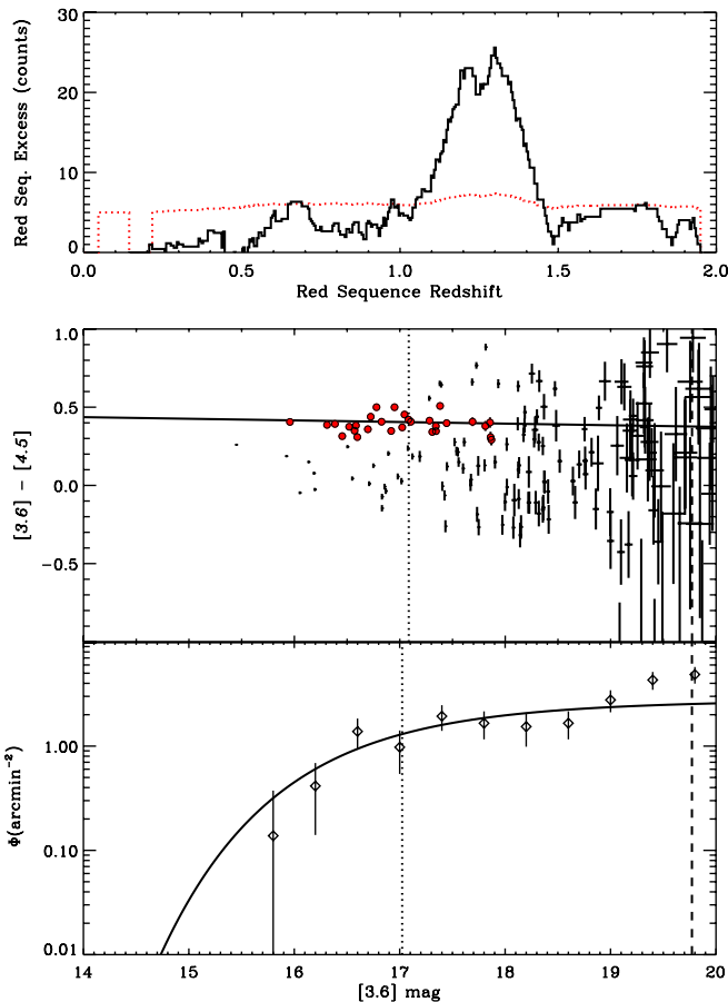
FIG. 2.— The cluster member finding for SPT-CL J0205-5829. The top panel shows the excess of surface density of galaxies (above background) consistent within 2\sigma of the SED model as a function of redshift. The RMS level of the overdensity is shown in dotted red. The peak overdensity is at z = 1.30 at 3.5\sigma above the background RMS. The middle panel shows the color-magnitude diagram of all objects within 2 arcminutes of the SPT center coordinates with red-filled black circles showing the selected galaxies from the passively-evolving model at z = 1.30 (black solid line) and brighter than m^* + 1 . The inferred model m^* is shown as a dotted vertical line and the [3.6] magnitude limit is shown as the dashed line. The bottom panel shows the Spitzer [3.6] galaxy luminosity function for SPT-CL J0205-5829. The dotted vertical line shows the best fit m^* in [3.6] , and the dashed line shows the [3.6] magnitude limit.
