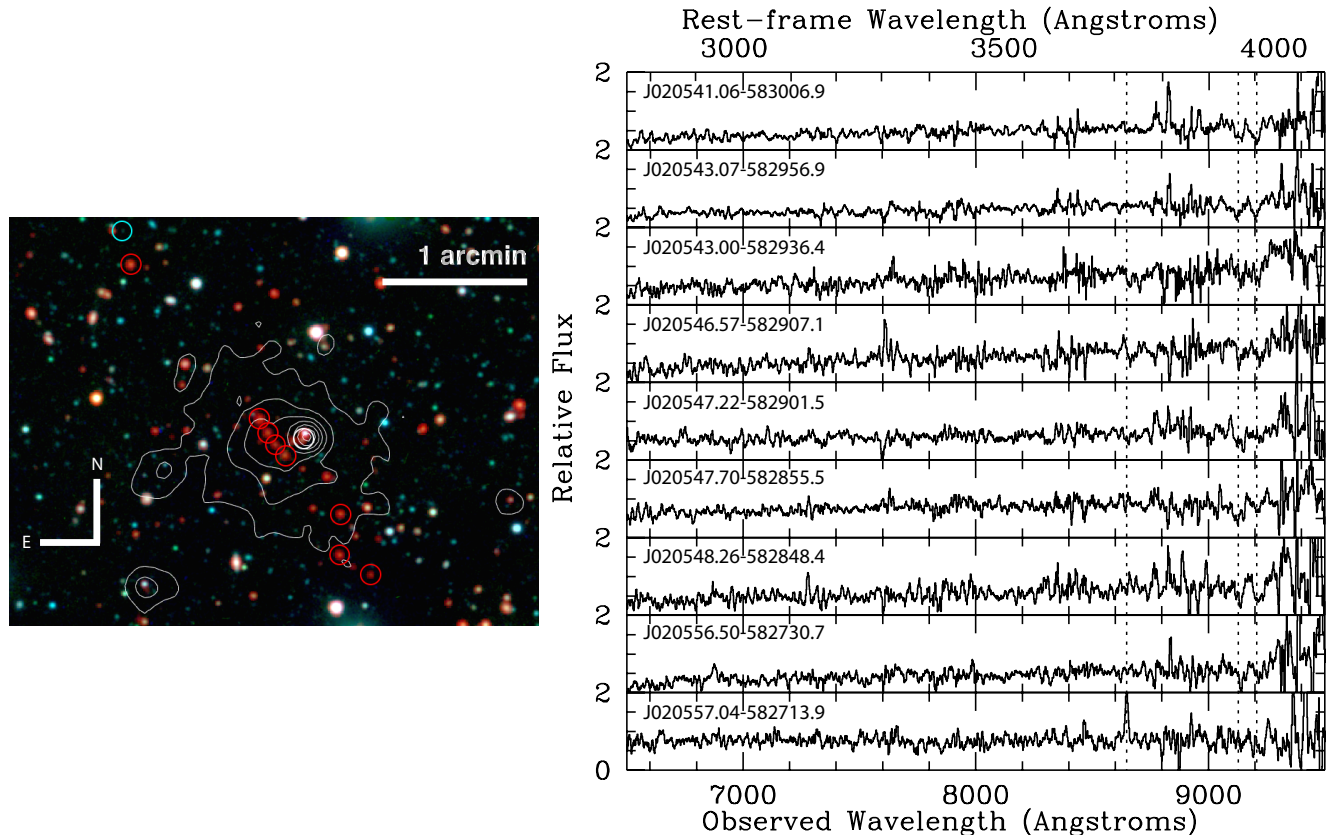
FIG. 3.— (Left) Optical (r/i) and Spitzer/IRAC [3.6] image showing the galaxies confirmed by spectroscopy and overlaid by the XMM-Newton X-ray contours. Cyan shows the [O II] detection shown to the right (bottom panel), and red shows the members identified with Ca H&K features shown to the right. The white circle shows the X-ray point source position. The frame subtends 4.5 \times 3.4 arcminutes. (Right) Spectra of all 9 member galaxies with the [O II] and Ca H&K features indicated in vertical dotted lines. Despite the long exposure time on Magellan, these features are faint due to the red color of passively galaxies.
