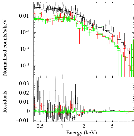
FIG. 5.— The X-ray spectrum of SPT-CL J0205-5829 (black: PN, green: MOS1, red: MOS2).
