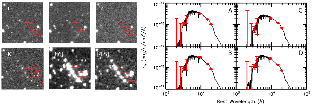
FIG. 4.— Best BC03 models for the four brightest galaxies in the central region of SPT-CL J0205-5829. The left panel shows thumbnails of 6 observed filters (r, i, z, K_s , [3.6], and [4.5]) in the central \sim 30'' from the brightest galaxy (A), with the four galaxies labeled in the K_s image. The right panels show the measured photometry in red with the best fit BC03 model for each overplotted.
