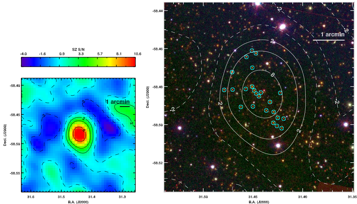
FIG. 1.— (Left) The filtered SPT-SZ significance map of SPT-CL J0205-5829. The negative trough surrounding the cluster is an artifact of the filtering of the time ordered data and maps. (Right) Color image from IMACS i , NEWFIRM K_S , Spitzer/IRAC [3.6], with SPT-SZ contours overlaid in white and [3.6]-[4.5] color-selected galaxies indicated in cyan.
