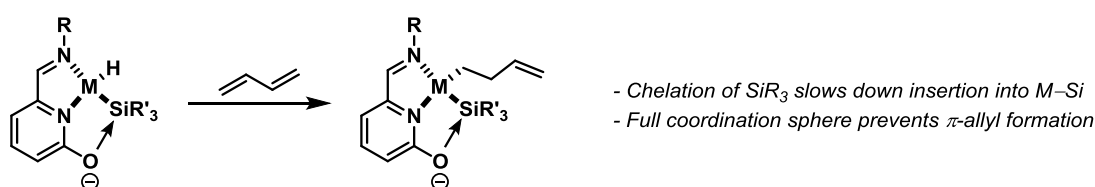
Scheme 17. Strategy for the 1,2-Selective Hydrosilylation of Conjugated Dienes
