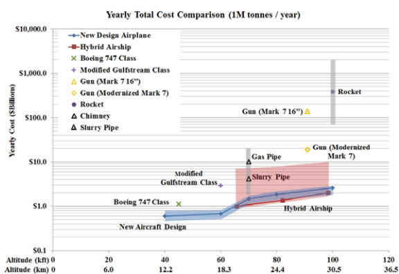
Figure 4. Comparison of yearly costs ($B) for geoengineering systems delivering 1 Mt yr -1 to the specified altitude. Shaded regions depict the range of uncertainty in cost estimates.
