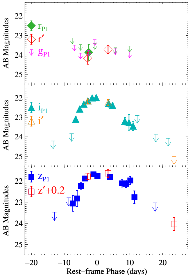
Figure 2. Multicolor optical light curves of PS1-10afx. Most of the data were obtained with PS1, but points marked r' , i' , or z' come from other telescopes (see Table 1). The r' i' z' photometry points near days -3 and +3 were taken contemporaneously with the optical spectra shown in Figure 4. Upper limits marked with arrows correspond to 3\sigma .
