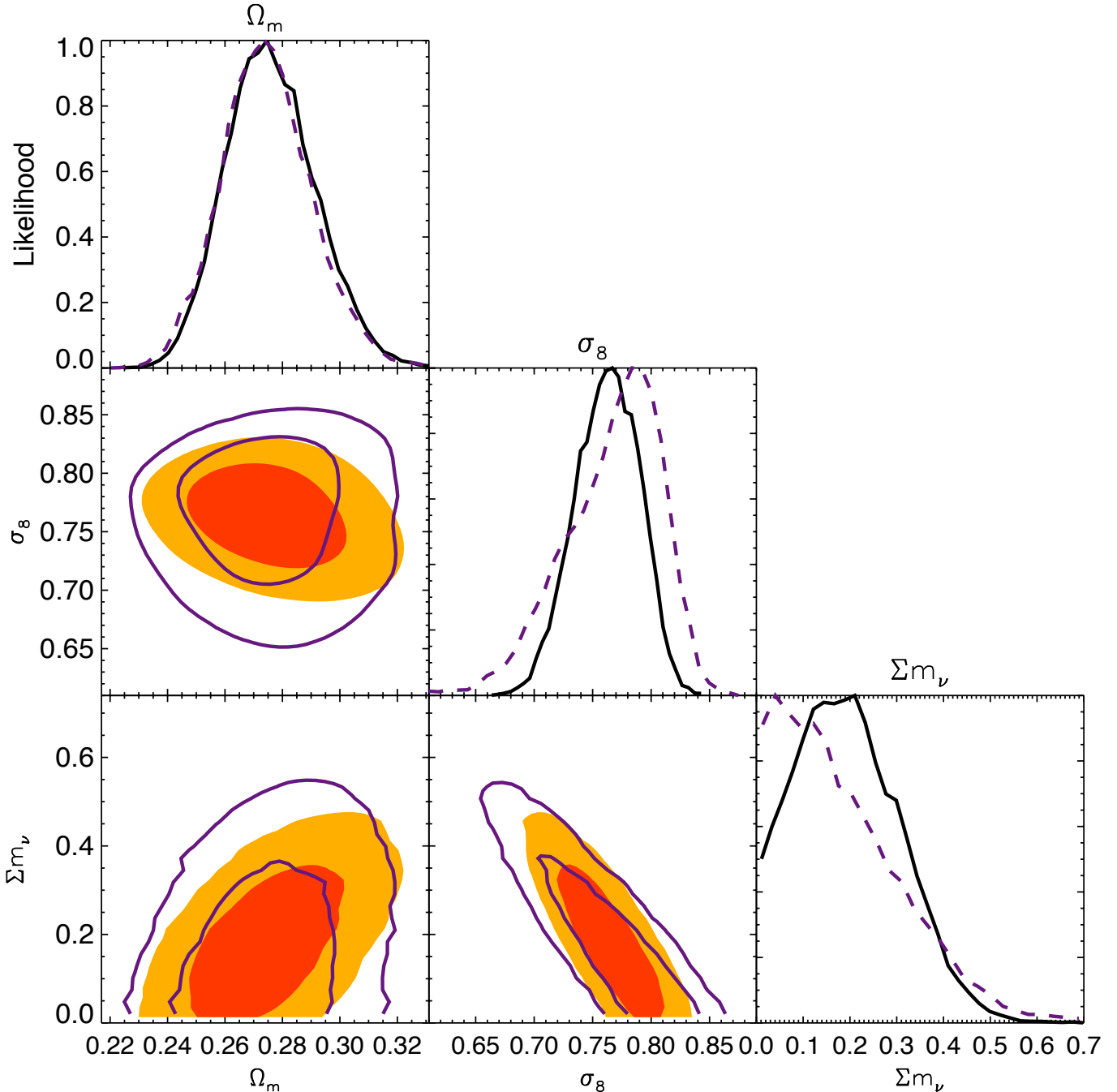
FIG. 7.— Assuming a \Lambda CDM + massive neutrino cosmology, the constraints on \Omega_m , \sigma_8 , and \Sigma m_\nu . The plots along the diagonal are the one-dimensional marginalized likelihood. The off-diagonal plots are the two-dimensional marginalized constraints showing the 68% and 95% confidence regions. We show the constraints for the CMB + BAO + H_0 (purple line contours and dashed lines), and CMB + BAO + H_0 + SPT CL (filled contours and black, solid lines) data sets. The SPT CL data leads to a small preference for positive neutrino masses with \Sigma m_\nu = 0.17 \pm 0.13 eV; the 95% CL upper limit on the neutrino masses is reduced from \Sigma m_\nu < 0.44 eV to \Sigma m_\nu < 0.38 eV.
