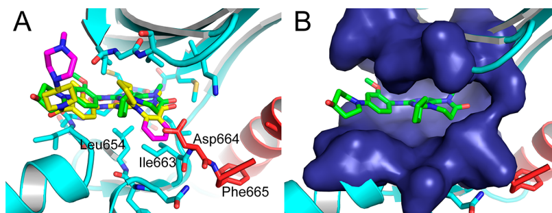
Figure 4. Comparison of binding of 25 to ERK5 with that of Mps1-IN-2 to TTK (PDB code 3H9F 32 ). (A) The TTK protein is colored cyan with the activation loop, and \alpha\text{C} helix is colored red. Inhibitor Mps1-IN-2 bound to TTK is colored green. The additional atoms present in 25 that are not present in Mps1-IN-2 are colored magenta, with the remainder of 25 colored yellow. (B) Surface of the TTK ATP-binding site around the inhibitor Mps1-IN-2.
